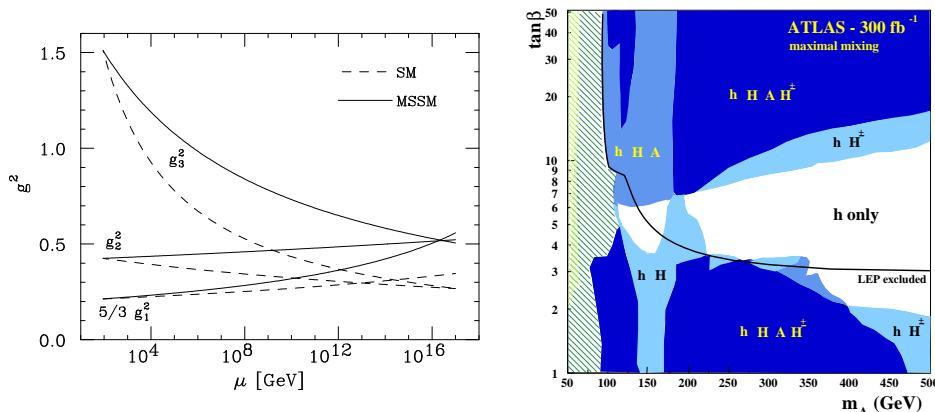
Fig. 2. The (non) unification of the three gauge couplings in the (SM) MSSM (left panel) and the reach of LHC for the MSSM Higgs [5] (right panel) .
