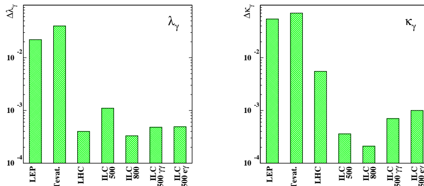
Fig. 7. A compilation of the reach of various colliders for the anomalous couplings of the photon [18].
