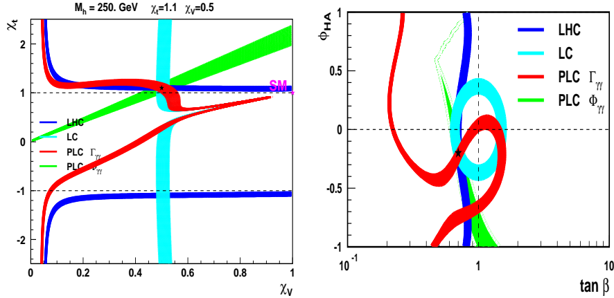
Fig. 6. The left panel shows the synergy between the LHC/ILC and the PLC in precise determination of the Higgs Boson couplings in a general 2 Higgs Doublet Model [16]. The star at (1,1) indicates the SM point and the 'star' at the centre of the plot corresponds to a particular set of parameters for the general 2HDM for which the light Higgs has a SM-like phenomenology. The plot in the right panel shows an example of the same synergy for the case of the Higgs Boson couplings in a CP violating 2HDM [17]. The plot shows that the measurements at all the three colliders will be needed to determine conclusively whether the CP-violating phase is nonzero.
