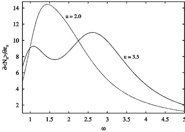
FIG. 3. The dependence of \partial\langle N_s\rangle/\partial\epsilon_s on \omega . For u=2.0 , there is only one peak corresponding to the DE to AE transition. For u=3.5 , there are two peaks corresponding to the DC to SAG to AC transitions.
