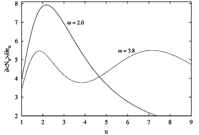
FIG. 4. The dependence of \partial\langle N_u\rangle/\partial\epsilon_u on u . For \omega=2.0 there is only one peak corresponding to the DE to DC transition. For \omega=3.8 , there are two peaks corresponding to the AE to AC to SAG transitions.
