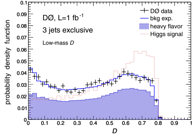
FIG. 1 (color online). Comparison of the low-mass likelihood distributions for the 3Tag data and background (bkg exp.) defined by Eq. (2). Every event has two entries, one for each jet pair. Black crosses refer to data, the solid line shows the total background estimate, and the shaded region represents the heavy flavor component ( bbb , bbc , and c\bar{c}b ). The distribution for a Higgs boson of mass 100 \text{GeV}/c^2 is also shown.
