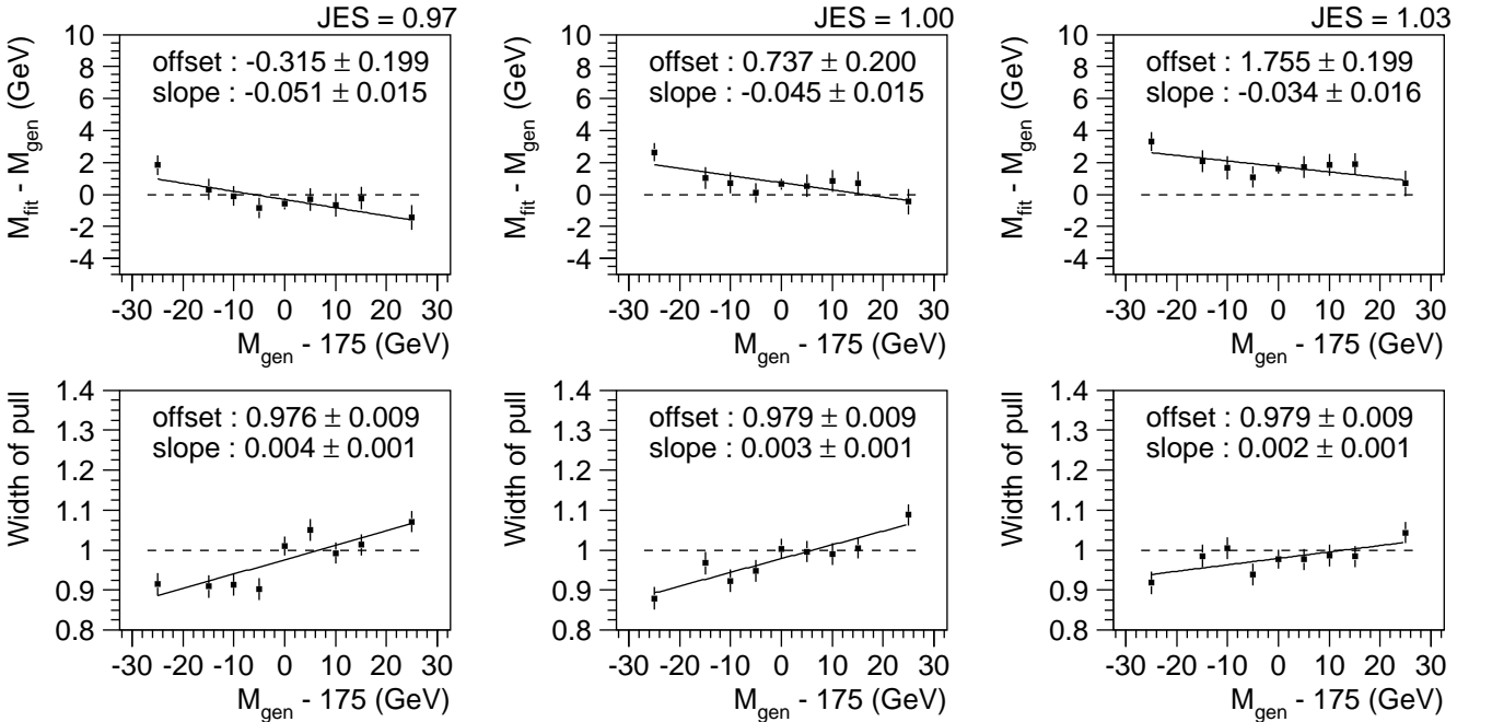
FIG. 6: The difference between the mean fitted mass M_{\text{fit}} and the generated top quark mass M_{\text{gen}} as a function of the generated top quark mass for a “true” JES of 0.97 (left), 1.00 (middle), and 1.03 (right), for the lepton+jets channel ( e + \mu combined). At a generated mass of 175 GeV, the mass bias changes by 1 GeV when the true JES is varied by \pm 3\% .
