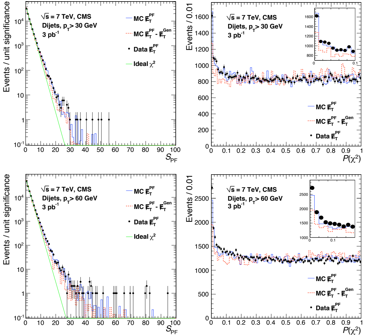
Figure 21: The \cancel{E}_T significance S_{\text{PF}} distributions (left) and the corresponding probability of \chi^2 , P(\chi^2) , distributions (right) for dijet event samples in data (points) and simulation (solid histograms) with 30 GeV (top) and 60 GeV (bottom) jet p_T thresholds. The dashed histograms show the simulation distributions with true \cancel{E}_T contributions, from physics and finite acceptance effects, subtracted event-by-event. The dotted line overlaid on the S_{\text{PF}} distributions shows a reference pure exponential function. Each inset expands the small P(\chi^2) region.
