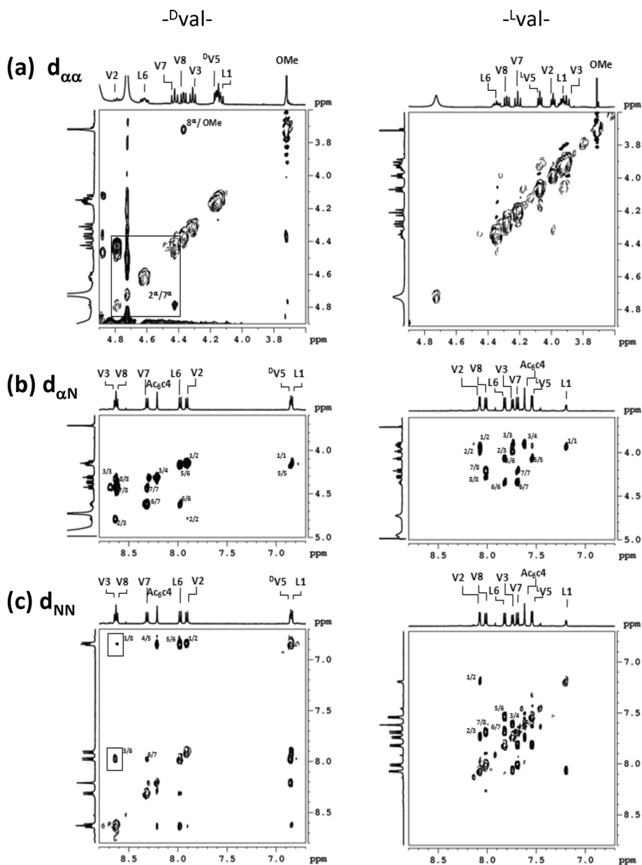
Fig. 3 Partial ROESY spectra of peptides 3 (right) and 4 (left). (a) C^\alpha proton region, (b) NH- C^\alpha H region, (c) NH-NH region. NOEs characteristic of hairpins ( d_{\alpha\alpha} 2/7 and d_{NN} 3/6) are boxed.
