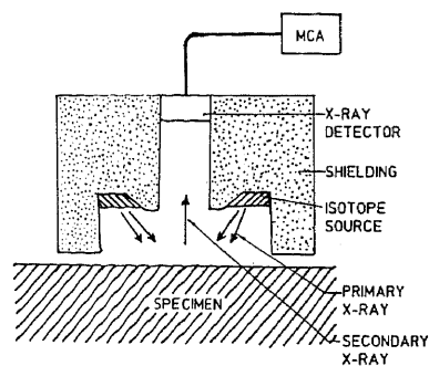
Figure 5. Schematic of portable XES system.
