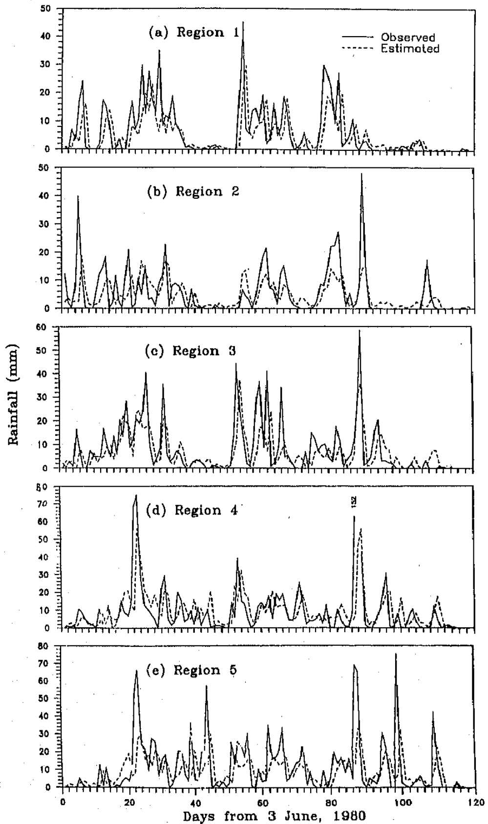
Figure 4. Time-series plots of observed and estimated daily areal rainfall (mm) using the QPF model for the monsoon season of 1980 over the five sub-regions of Narmada Catchment.
