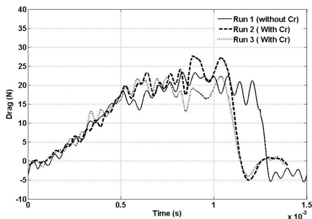
FIG. 2. Measured drag signals for the 60° apex angle blunt cone with and without chromium plating in Mach 8 hypersonic flow with a specific enthalpy of 2.3 MJ/kg.
