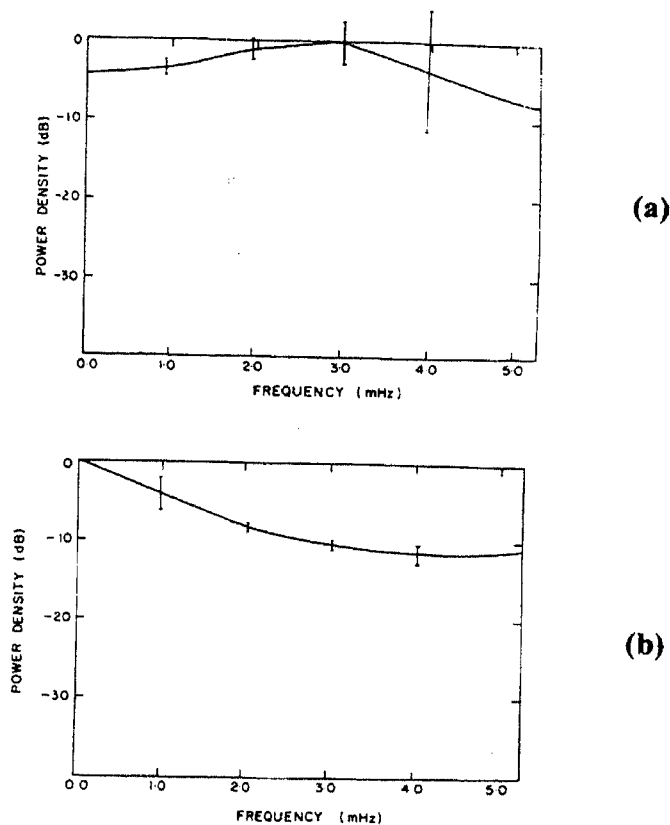
Figure 4a-b. a. Spectrum of solar brightness temperature at 2.8 GHz before the 1st contact on 16 February 1980. b. Spectrum of solar brightness temperature at 2.8 GHz after the 4th contact on 16 February 1980.
