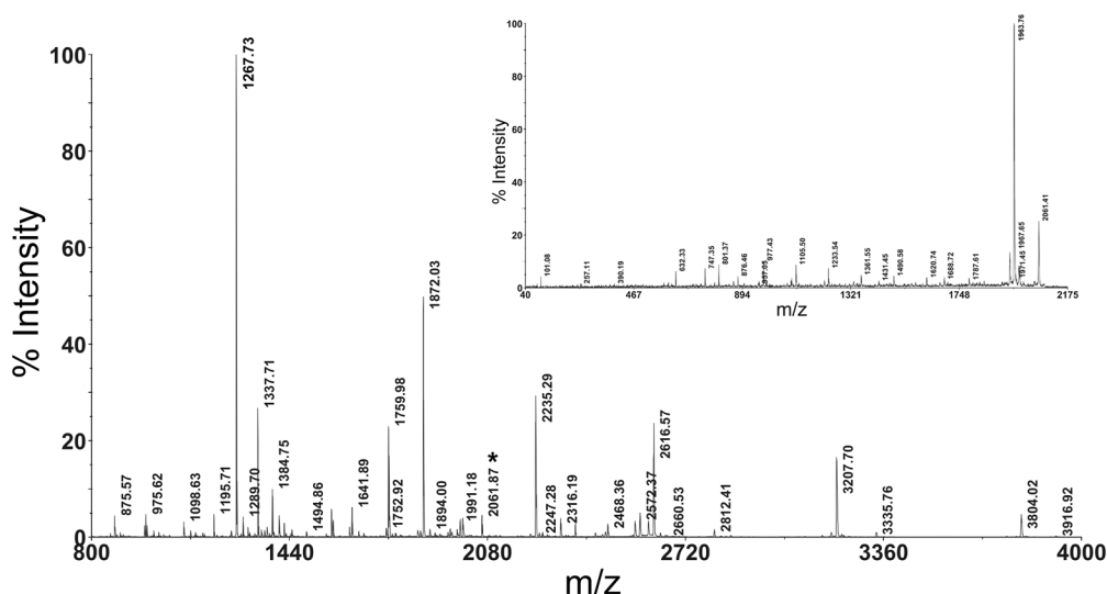
Figure 6. The trypsin digest of the protein casein spiked with the phosphopeptide. The inset shows the CID mass spectrum of the monophosphopeptide. The symbol (*) in the mass spectrum indicates the spiked peptide.
