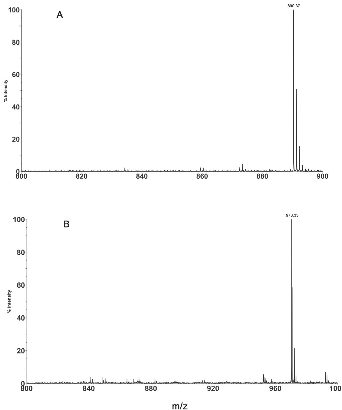
Figure 1. MALDI-TOF mass spectra of the peptides E8G (panel A ) and E8Gp (panel B ) recorded in the reflector mode using HCCA as matrix. The isotopic peaks of the peptides are also shown.
