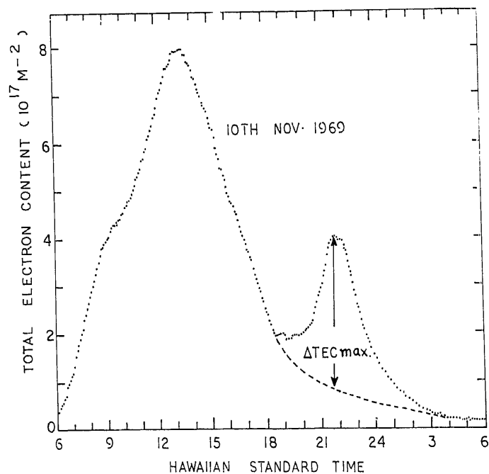
Figure 1. Diurnal variation of TEC at Hawaii on a solar maximum day illustrating the occurrence of a strong night-time TEC enhancement.
