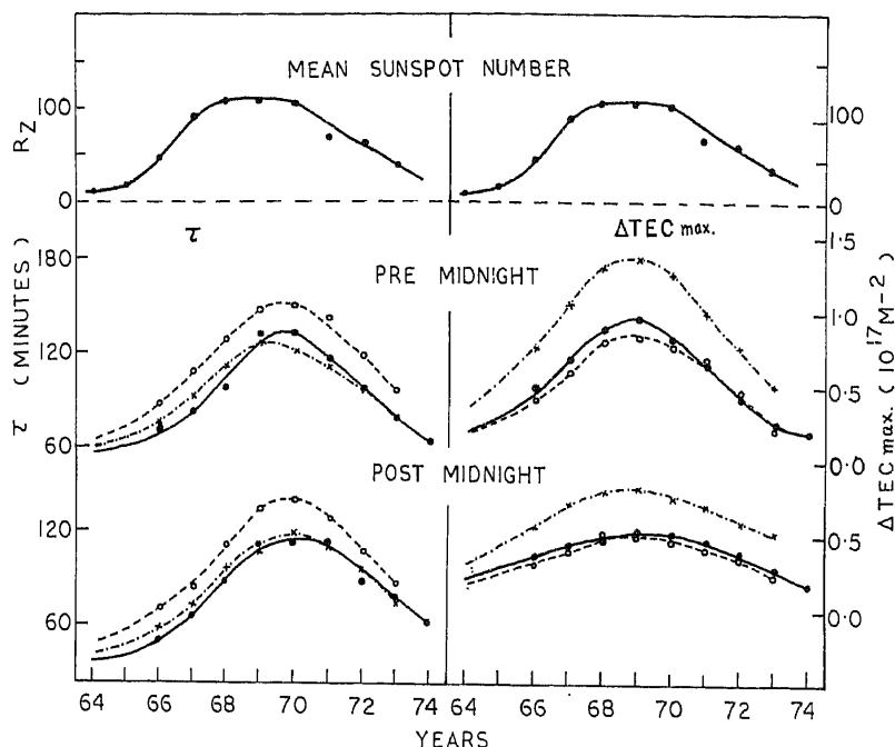
Figure 6. Solar cycle variation of yearly mean sunspot number and seasonal mean \tau and \Delta\text{TEC}_{\text{max}} of pre-midnight and post-midnight TEC enhancements for the three seasons (●---● winter, ○---○ summer and ×---× equinox) at Hawaii.
