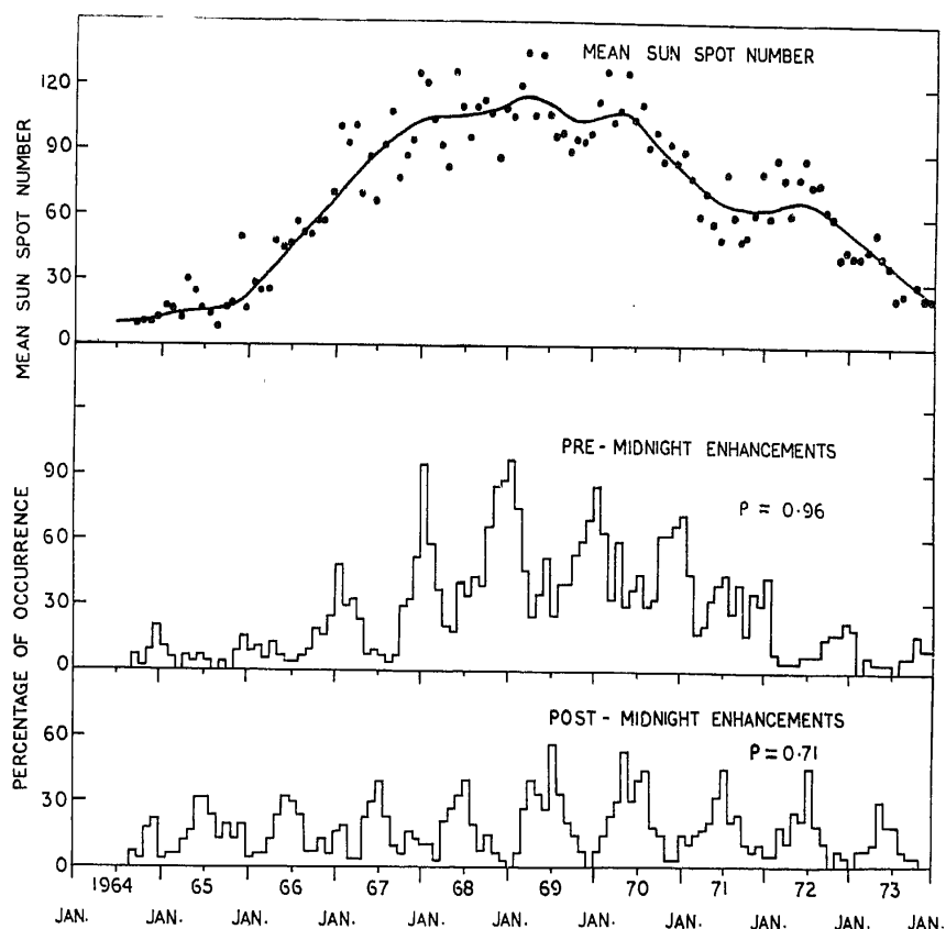
Figure 2. Dependence of the frequency of occurrence(%) of pre-midnight and post-midnight TEC enhancements on solar activity during the period 1964-73 at Hawaii. Top portion of the figure gives the variation of monthly mean sun spot number.
