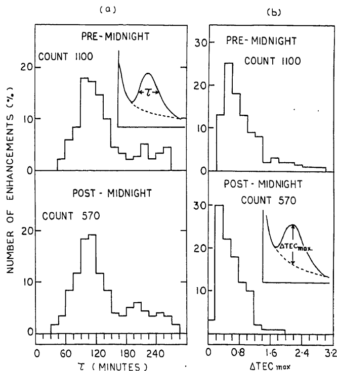
Figure 4. Distribution of (a) the half-amplitude duration ( \tau ) and (b) the amplitude ( \Delta\text{TEC}_{\text{max}} ) of pre-midnight and post-midnight TEC enhancements at Hawaii.
