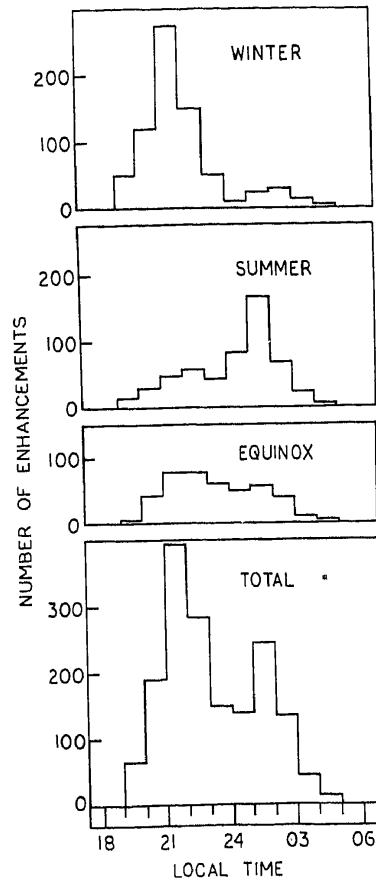
Figure 3. Distribution of the occurrence time of the peak of TEC enhancement at Hawaii for each season and for all the data combined.
