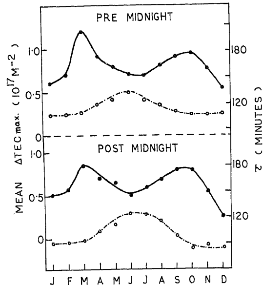
Figure 5. Monthly mean variation of \tau (○---○) and \Delta\text{TEC}_{\text{max}} (●---●) of pre-midnight and post-midnight TEC enhancements at Hawaii.
