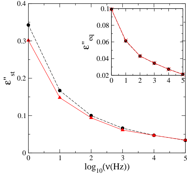
FIG. 2: The best fit values of \epsilon''_{\text{st}} for the curves in fig. 1 vs. frequency \nu(\text{Hz}) as obtained with the present work (solid line) and the corresponding results of Ref. [5] (dashed). The inset shows the best fit \epsilon''_{\text{eq}} with frequency \nu respectively from the present work and Ref. [5].
