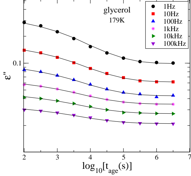
FIG. 1: \epsilon''(t_{\text{age}}) data for glycerol at 179^\circ\text{K} vs. t_{\text{age}} (in sec) at the frequencies displayed in the inset. Solid lines correspond to the best fits using the modified KWW form with \tau_{\text{age}}(t_{\text{age}}) determined from eqn. (4).
