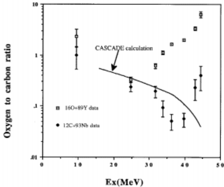
Figure 1. Ratio of oxygen to carbon yields versus excitation energy.
