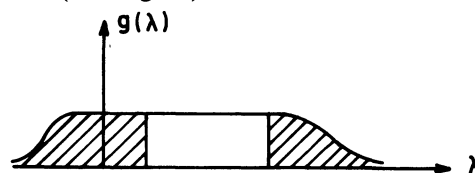
FIG. 2. — Density function of the eigenvalue spectrum of D . Hachured regions correspond to localized states.
