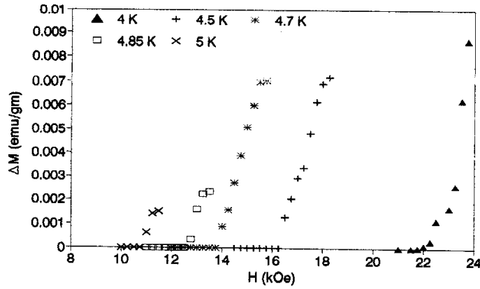
Figure 10. Field dependence of the rise in equilibrium magnetization for a polycrystalline \text{CeRu}_2 sample at various temperatures [94].
