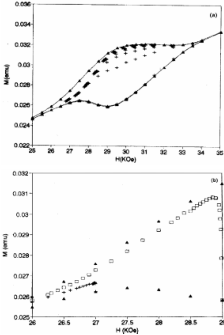
Figure 7. Forward legs of the minor hysteresis loops (MHL): (a) starting at H = 27, 27.5, 28, 28.5, 29, 29.5, 30, 30.5, 31, 31.5 and 32.5 kOe with the maximum change in field (\Delta H)_{\max} = 250 Oe [(+) MHLs; ( \blacktriangle ) envelope curve]; (b) starting at H = 27 kOe (+) and 29 kOe ( \blacktriangle ) and reducing the field to 26 kOe. All these MHLs are initiated from the lower envelope curve [72].
