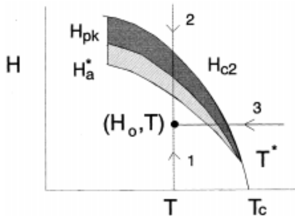
Figure 8. Schematic phase diagram of the superconducting mixed state of \text{CeRu}_2 . Paths indicated by 2 and 3 corresponds to isothermal field reduction and field cooling through the high-entropy phase. A critical point is indicated at T^* , above which this phase does not exist [93].
