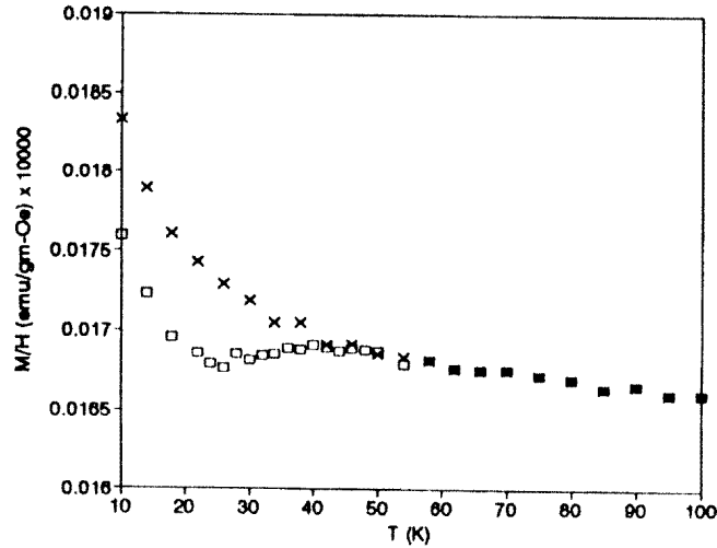
Figure 3. Magnetic susceptibility ( M/H ) vs temperature ( T ) plot of CeRu_2 single crystal sample, with external field ( H ) being kept constant at 500 Oe. \square stands for zero field cooled and X for field cooled susceptibility [20].
