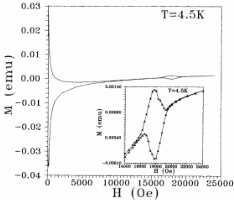
Figure 5. Magnetization ( M ) vs field ( H ) plot for a polycrystalline sample of \text{CeRu}_2 at T = 4.5 K. Inset shows enlarged M-H plot near H_{C2} to highlight the peak-effect.
