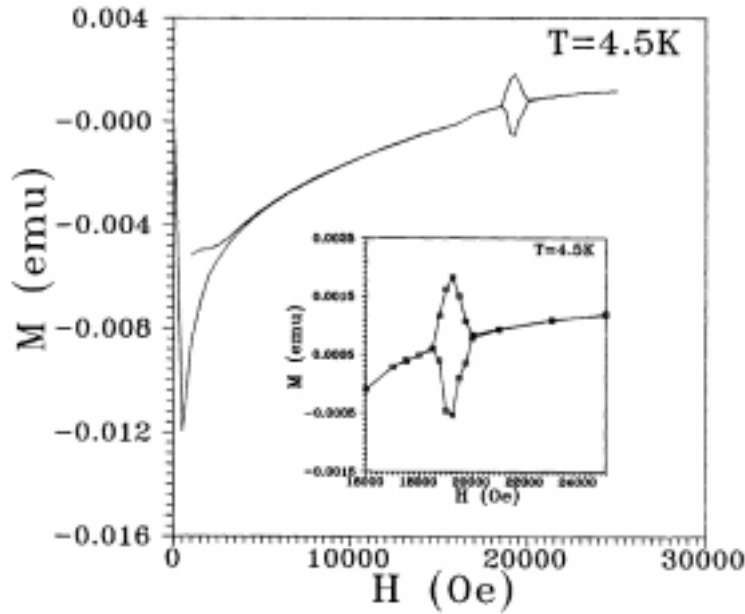
Figure 6. Magnetization ( M ) vs field ( H ) plot for a single crystal sample of CeRu 2 at T = 4.5 K. Inset shows enlarged M-H plot near H_{C2} to highlight the peak-effect.
