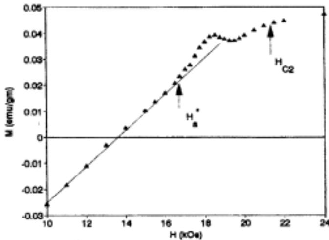
Figure 9. Equilibrium magnetization ( M_{\text{eq}} ) versus field ( H ) plot at T = 4.5 K for a polycrystalline \text{CeRu}_2 sample [73].
