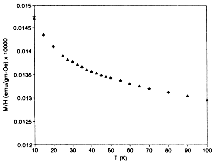
Figure 2. Magnetic susceptibility ( M/H ) vs temperature ( T ) plot of \text{CeRu}_2 single crystal sample, with external field ( H ) being kept constant at 5 kOe. \blacktriangle stands for zero field cooled and + for field cooled susceptibility [20].
