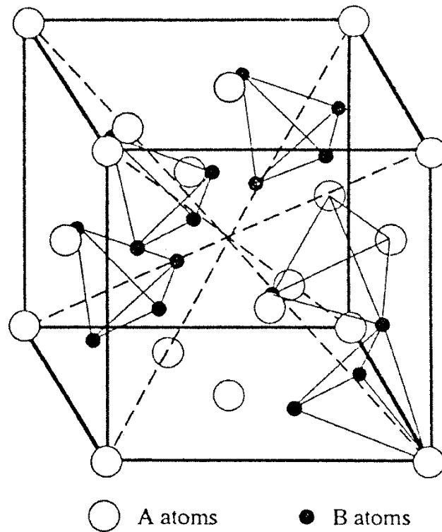
Figure 1. Crystal structure of C15 Laves phase.
