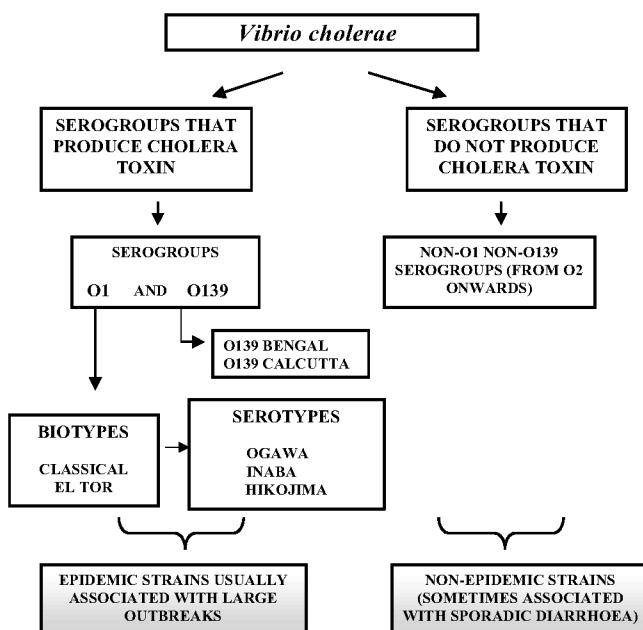
Figure 1. Classification of Vibrio cholerae serogroups into epidemic and non-epidemic groups is shown; the respective biotypes within a serotype are also represented. The O1 and O139 serogroups are currently the only ones associated with epidemic cholera.
