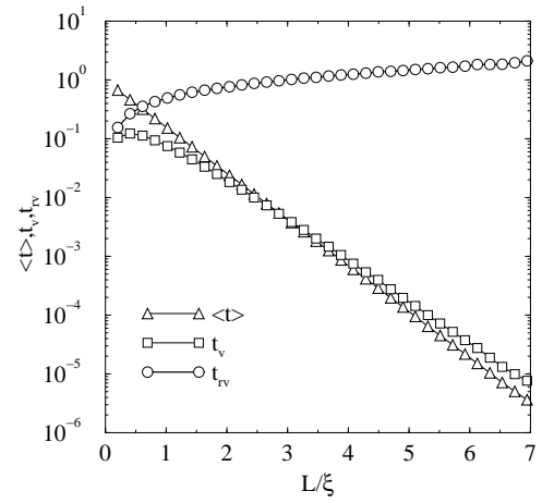
FIG. 3. Average transmission coefficient \langle t \rangle , variance of t ( t_v ) and relative variance of t ( t_{rv} ) as a function of L/\xi for fixed disorder W = 1.0 and absorption \alpha = 0.01 .
