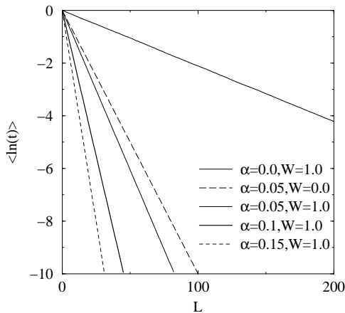
FIG. 1. Average of logarithm of transmission coefficient t versus length L for different values of absorption strength \alpha and disorder strength W as indicated in the figure.
