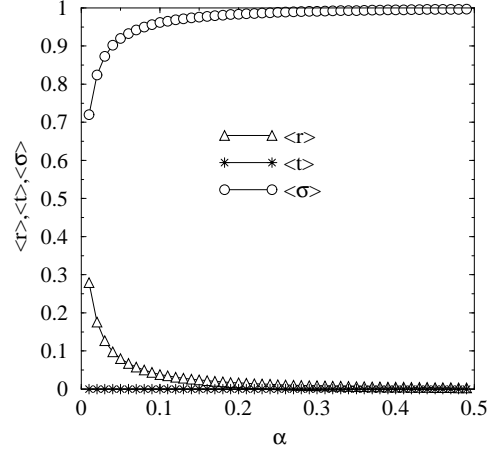
FIG. 8. Average value of reflection coefficient ( \langle r \rangle ), transmission coefficient ( \langle t \rangle ) and absorption ( \langle \sigma \rangle ) versus absorption strength \alpha for W = 1.0 and L/\xi = 10 .
