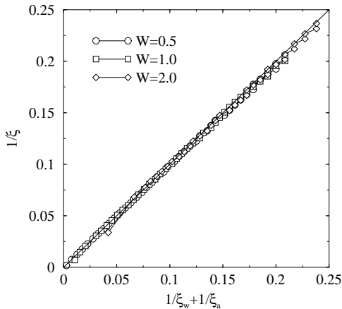
FIG. 2. 1/\xi versus 1/\xi_w + 1/\xi_a , where \xi_w is the localization length for non-absorptive disordered system, \xi_a is the localization length for ordered absorptive system and \xi is the localization length for absorptive disordered system.
