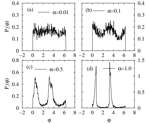
FIG. 9. Stationary distribution of phase of reflected wave for fixed disorder strength W = 1.0 and different values of absorption \alpha .
