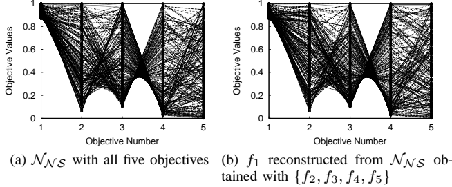
Fig. 14. Storm drainage problem: Parallel coordinate plots (normalized), corresponding to one run of NSGA-II.
