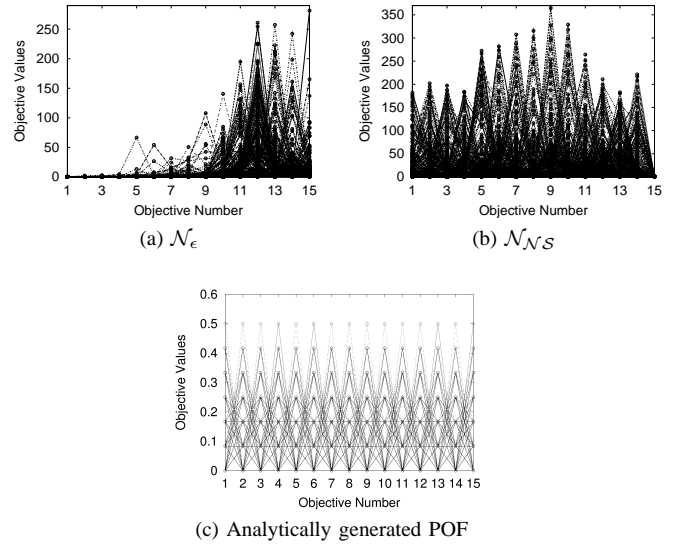
Fig. 9. DTLZ1(15): Parallel coordinate plots for \mathcal{N}_\epsilon , \mathcal{N}_{NS} (one run) and analytically generated POF.
