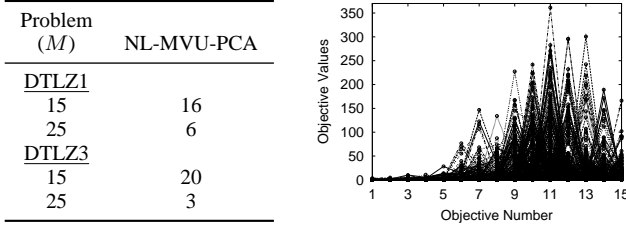
(a) These results indicate the successful cases in 20 random runs (b) Parallel coordinate plot of DTLZ1(15), for one run.
