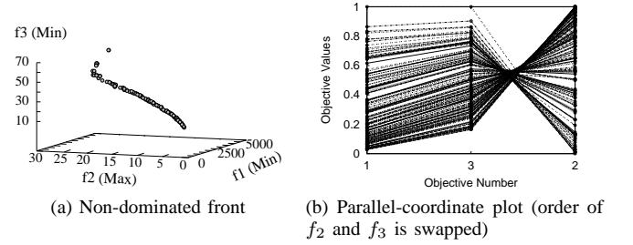
Fig. 13. Multi-speed gearbox design problem. The plots correspond to one run of NSGA-II.
