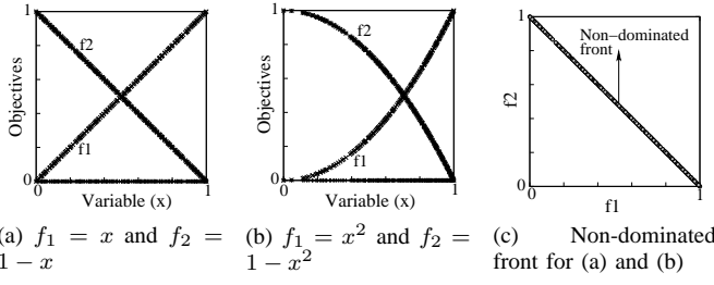
Fig. 2. Illustration: (a) Two linear objectives, and (b) Two identically nonlinear objectives, resulting in (c) a linear non-dominated front. x \in [0,1] .
