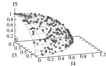
Fig. 8. DTLZ5(3, 5): Illustrating that the \mathcal{N}_{\mathcal{N}S} (one run) obtained for the reduced problem, \mathcal{F}_T = \{f_3, f_4, f_5\} , conforms with the true POF.
