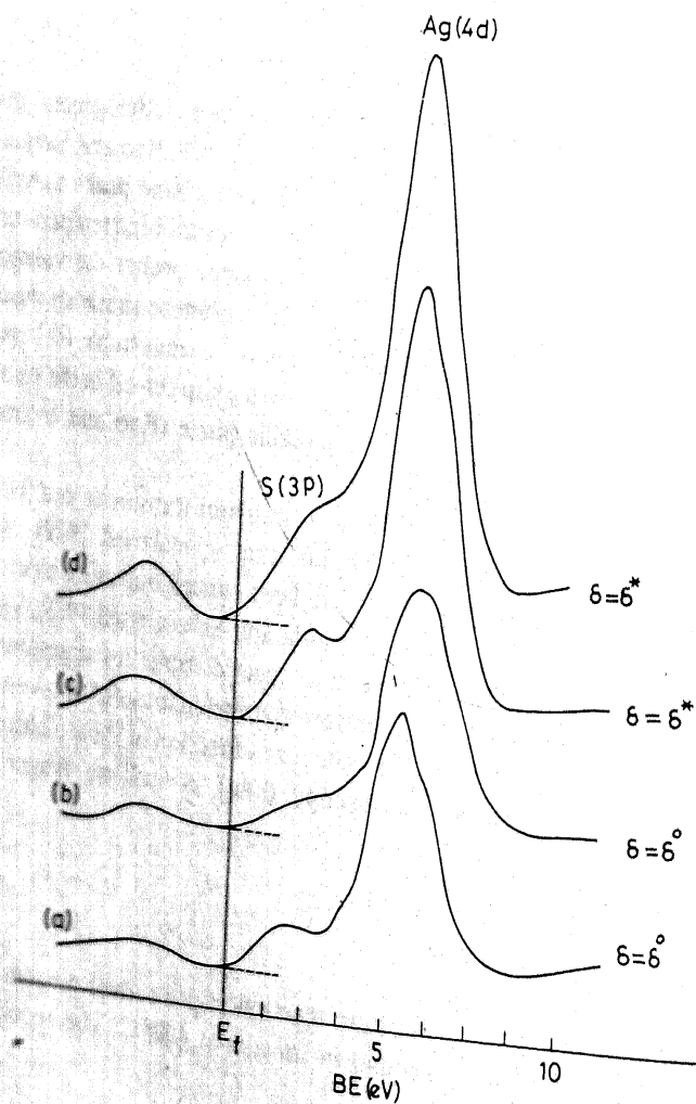
Figure 1. X-ray photoelectron spectra of the valence band in: (a) Ag 2+ \delta S ( \delta = \delta^{\circ} ) at 295 K; (b) Ag 2+ \delta S ( \delta = \delta^{\circ} ) at 473 K; (c) Ag 2+ \delta S ( \delta = \delta^* ) at 295 K; and (d) Ag 2+ \delta S ( \delta = \delta^* ) at 473 K.
