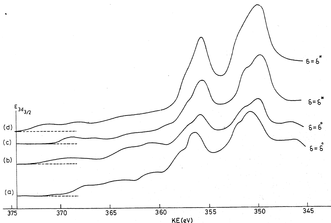
Figure 2. X-ray induced Auger electron spectra of the Ag(M_{45}N_{45}N_{45}) region in: (a) Ag_{2+\delta}S ( \delta = \delta^\circ ) at 295 K; (b) Ag_{2+\delta}S ( \delta = \delta^\circ ) at 473 K; (c) Ag_{2+\delta}S ( \delta = \delta^* ) at 295 K; and (d) Ag_{2+\delta}S ( \delta = \delta^* ) at 473 K.
