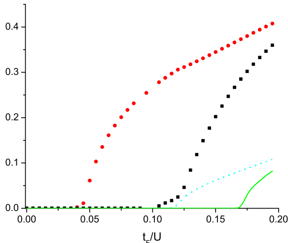
FIG. 7: (Color online) Plot of \Delta and Z for \mu/U = 0.4 , \eta = 4 and \lambda = 0 and \lambda = 0.3 . All symbols have the same meaning as Fig. 5. The plot serves as an illustration that repulsive interaction between bosons and fermions can enhance metal/superfluid transitions.
