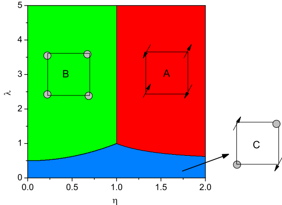
FIG. 2: (Color online) Possible ground states A, B and C that results from lifting the classical degeneracy of the ground states (n_0^B, n_0^F) = (1, 0) and (0, 1) due to quantum fluctuations. Notice that the antiferromagnetic ordering of state C is different from state A and is a consequence of very weak next nearest neighbor hopping. Similar states will result when the degeneracy of the states (2, 1) and (1, 2) is lifted.
