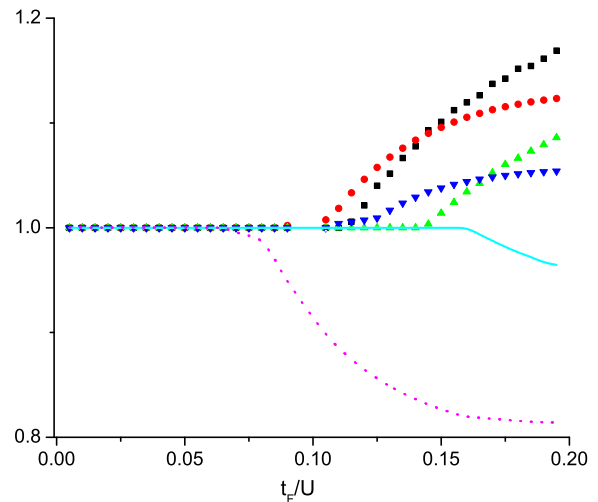
FIG. 6: (Color online) Plot of the average densities \bar{n}_B and \bar{n}_F for the bosons and Fermions for \mu/U = 0.7 and \eta = 5 . The deviation of the densities from their quantized values in the Mott state signals the onset of metal-insulator transition for fermions and superfluid-insulator transition for the bosons. The symbols are as follows: black square and red circle ( \bar{n}_B and \bar{n}_F respectively for \lambda = 0 ), green uptriangle and blue downtriangle ( \bar{n}_B and \bar{n}_F respectively for \lambda = 0.3 ), magenta dotted line and cyan solid line ( \bar{n}_B and \bar{n}_F respectively for \lambda = 0.5 ).
