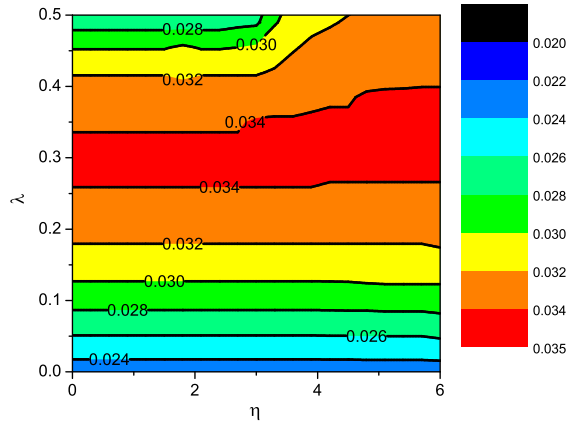
FIG. 8: (Color online) Plot of t_B^c/U as a function of \eta and \lambda for \mu/U = 0.7 . For small \eta , the fermions remain in the Mott state when the superfluid-insulator transition of the bosons takes place whereas for large \eta they have already undergone a metal-insulator transition.
