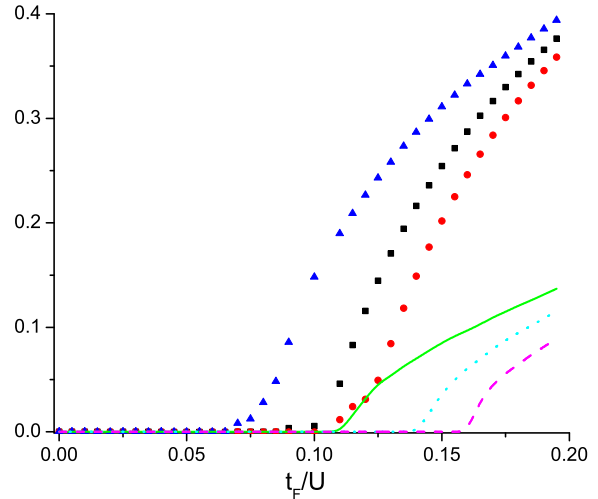
FIG. 5: (Color online) Plot of the order parameter \Delta and Z for \mu/U = 0.7 and \eta = 5 . Non-zero values of \Delta / Z signals superfluid/metal-insulator transition for the Boson/fermions. The symbols are as follows: black squares and green solid line ( \Delta and Z respectively for \lambda = 0 ), red circles and cyan dotted line ( \Delta and Z respectively for \lambda = 0.3 ), and blue triangles and magenta dashed line ( \Delta and Z respectively for \lambda = 0.5 ).
