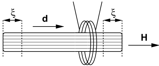
FIG. 4. Schematic experimental setup to measure magnetic susceptibility of the edge states localized at the ends of the chains.
