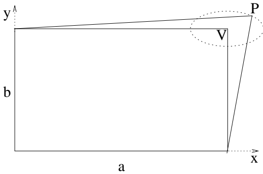
FIG. 1. A deformation of a rectangle into a quadrilateral. The vertex V = (a, b) is moved to the point P = V + (\delta x, \delta y) = V + ab(\alpha, \beta) . We consider an experiment where P is moved around the elliptic path shown in the figure.
