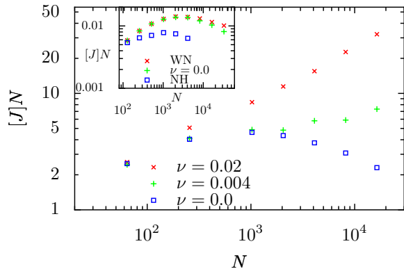
FIG. 4: Plot of heat current versus system size, for the disordered anharmonic chain, for different values of \nu . The data in the inset, corresponds to parameters (T_L, T_R) = (0.001, 0.0005) with Gaussian white bath for \nu = 1 (WN) and \nu = 0 , and Nose-Hoover bath (NH) for \nu = 1 .
