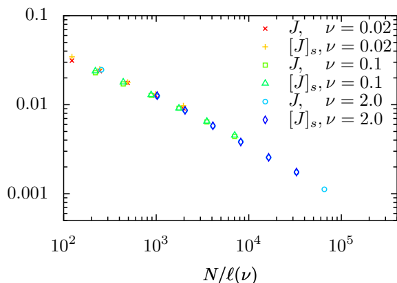
FIG. 5: Plot of scaled heat current versus scaled system size, for the binary-mass ordered ( J ) and disordered ( [J]_s ) anharmonic chains, for different values of \nu .
