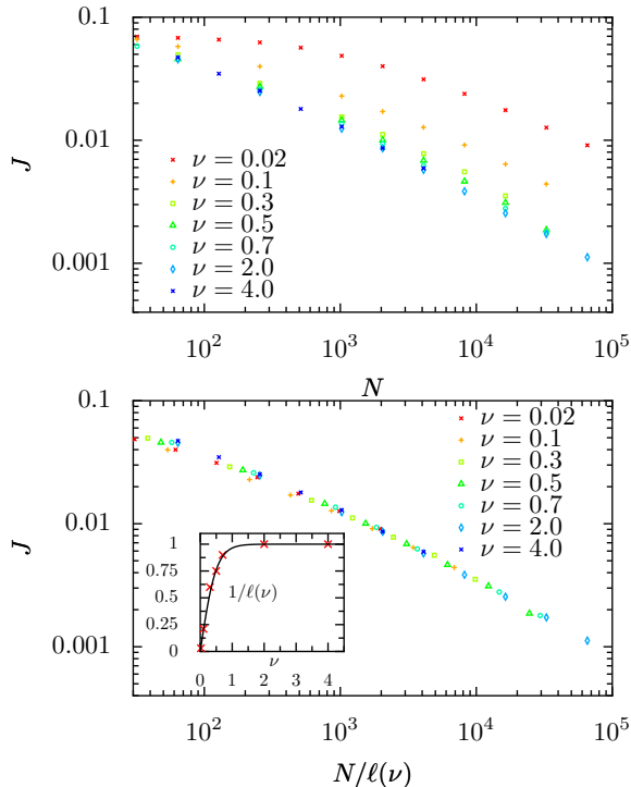
FIG. 2: Plot of the heat current J versus system size for the binary mass ordered chain, for different values of \nu and with the mass ratio A = 1.5 (a). Fig (b) shows the same data plotted with a scaled x -axis.
