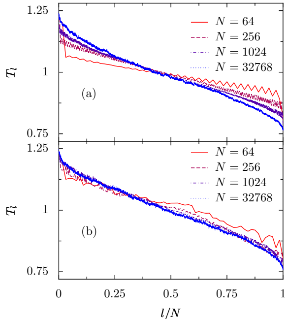
FIG. 3: Plot of the temperature profiles in the (a) ordered and (b) disordered lattices for \nu = 0.1 and for different system sizes.
