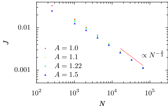
FIG. 1: Plot of the heat current J versus system size in the binary mass ordered chain for different values of the mass ratio A = 1.0, 1.1, 1.22 and 1.5 .
