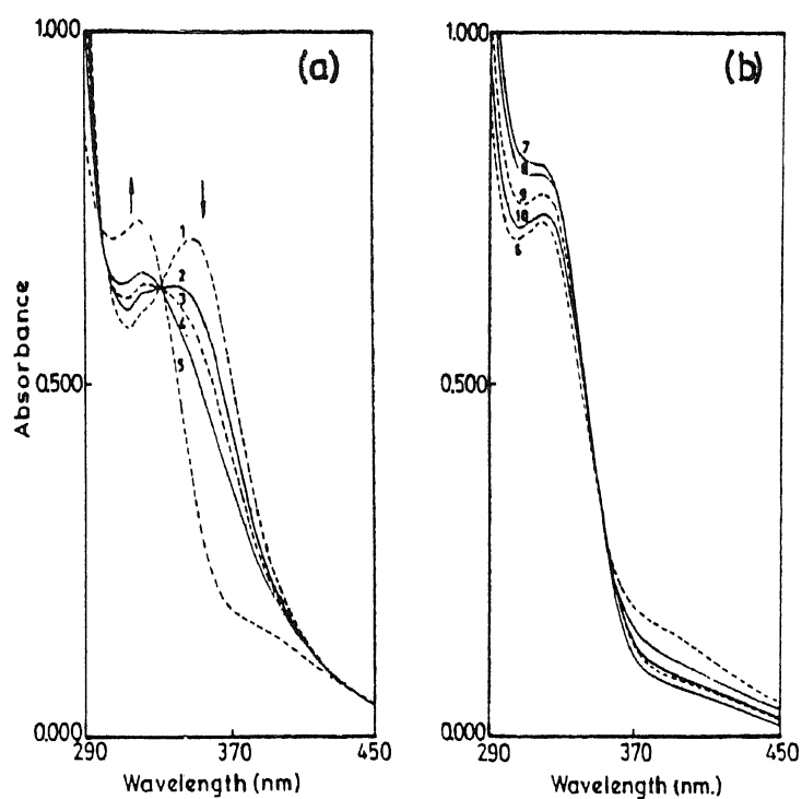
Figure 2. Absorption spectra as a function of time: (a) of the mixture of 1 + \text{H}_2\text{O}_2 + \text{HCl} ; (b) of that in (a) + \text{Et}_4\text{NBr} . Spectra are recorded at: (1) 0; (2) 2; (3) 5; (4) 8; and (5) 20 min in case of (a); and (6) 0; (7) 2; (8) 9; (9) 14 and (10) 20 min in case of (b).
