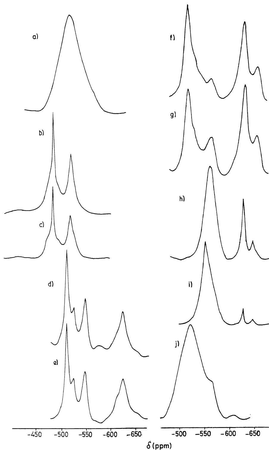
Figure 4. ^{51}\text{V} NMR spectra of the reaction between complex 2 and \text{H}_2\text{O}_2 and KBr as a function of time (a) Complex 2 in dmf; (b) a + \text{HClO}_4 , 11 min; (c) 21 min; (d) c + \text{H}_2\text{O}_2 , 1 min; (e) 10 min; (f) 30 min; (g) f + KBr, 1 min; (h) 10 min; (i) 30 min and (j) 60 min.
