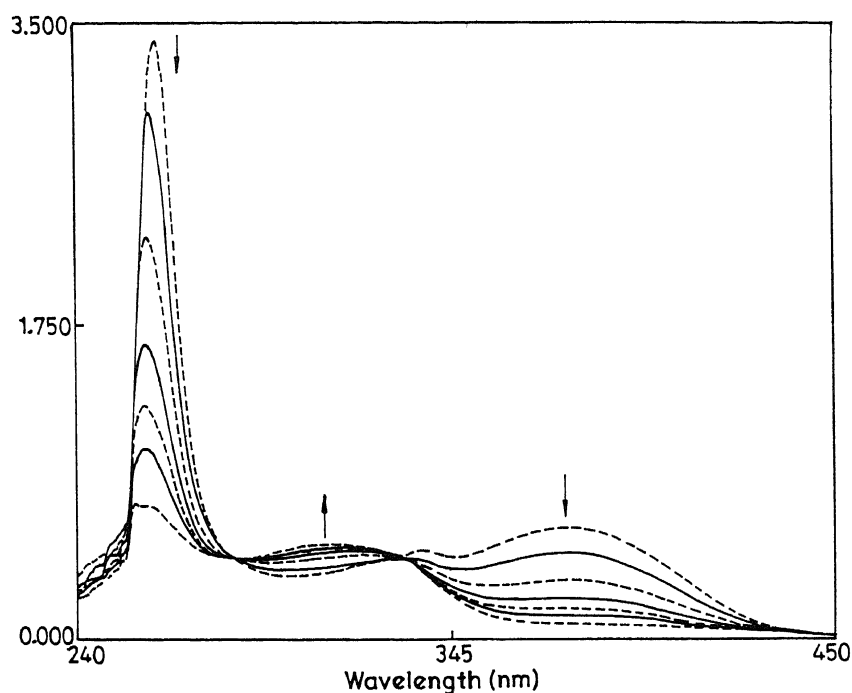
Figure 1. UV-VIS spectra of a reaction mixture of 2 and \text{H}_2\text{O}_2 (1:8) as a function of time over a period of 30 min.
