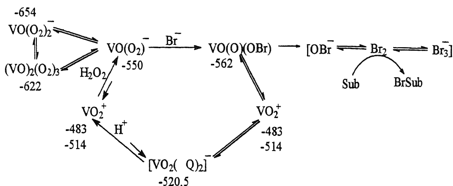
Scheme 2. Experimentally observed steps during the bromination reaction of 2 . Correct species among those shown in brackets is not fully conformed. The numerical values indicate ^{51}\text{V} NMR chemical shifts.
