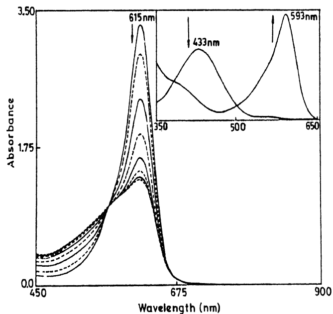
Figure 3. Absorption spectra of bromination of (a) Xylene cyanole by \text{cis-VO}_2^+ generated from a mixture given in figure 2(b), Inset: bromination of phenol red by the same reaction mixture.
