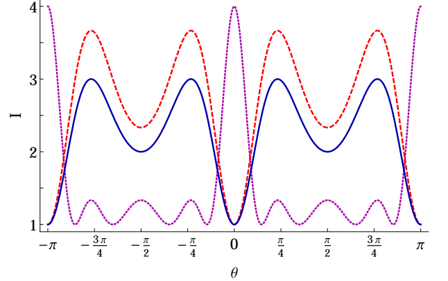
FIG. 9: (Color online) Plot of the angular dependent intensity of the initial anti-symmetric state |W_{2,1}^-\rangle (striped) and the anti-symmetric state |\tilde{W}_{2,1}^-\rangle (solid) compared to the symmetric W-state |W_{2,1}\rangle (dotted); kd = \frac{3}{2}\pi and I is given in units of the intensity produced by a one atom system.
