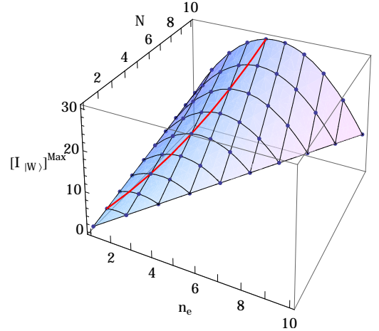
FIG. 4: (Color online) Pointplot of the maximum of I_{|W_{n_e, N-n_e}\rangle} as a function of n_e and N = n_e + n_g (the surface serves only to guide the eye). [I_{|W_{N/2, N/2}\rangle}]^{\text{Max}} , given in units of the intensity produced by a one atom system, is highlighted by the solid line.
