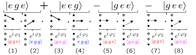
FIG. 8: (Color online) Quantum paths of the anti-symmetric state |W_{2,1}^-\rangle . Black circles denote atoms in the excited state and white circles denote atoms in the ground state. The middle row depicts the different quantum paths. The lower row displays the final states of the atoms and the phases accumulated by the photon due to different quantum paths. Quantum paths leading to constructive interference are denoted by solid arrows and quantum paths leading to destructive interference are depicted by dashed arrows. See text for details.
