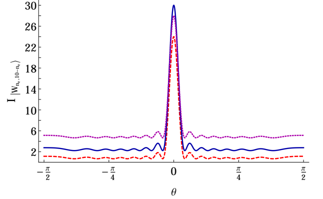
FIG. 6: (Color online) Intensity distribution of the state |W_{n_e, 10-n_e}\rangle for N = 10 and different numbers of excited atoms n_e ( n_e = 3 striped, n_e = 5 solid, n_e = 7 dotted); kd = \frac{3}{2}\pi and I_{|W_{n_e, 10-n_e}\rangle} is given in units of the intensity produced by a one atom system.
