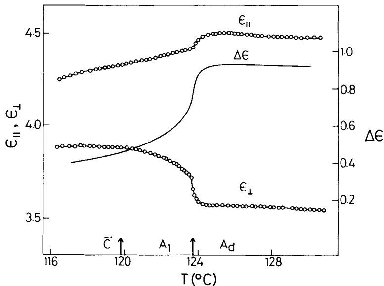
FIGURE 7 Temperature variation of the principle dielectric constants ( \epsilon_{||} , \epsilon_{\perp} ) and the dielectric anisotropy ( \Delta\epsilon ) near the A_d - A_1 transition in the DB NO 2 mixture.
