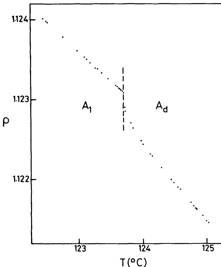
FIGURE 6 Temperature variation of the density ( \rho ) in the vicinity of the A_d - A_1 transition in the DBNO_2 mixture.
