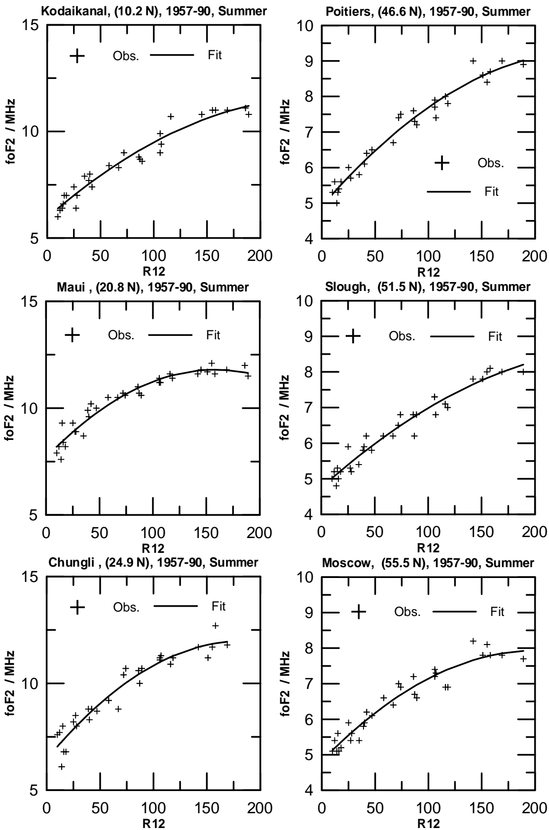
Fig. 1. Shows the plots of observed monthly median noon f_oF2 values against R12 during summer. The regression fits are shown as solid line. The left panels show low latitude stations, while the mid-latitude stations are shown on the right panel of the figure.
