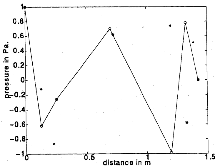
Figure 4. Comparison of FEM predictions (*) for a square pipe model of length 1.445 m, side 0.05 m and a segment length 0.7 times the wavelength with analytical solution (o) given by (25).
