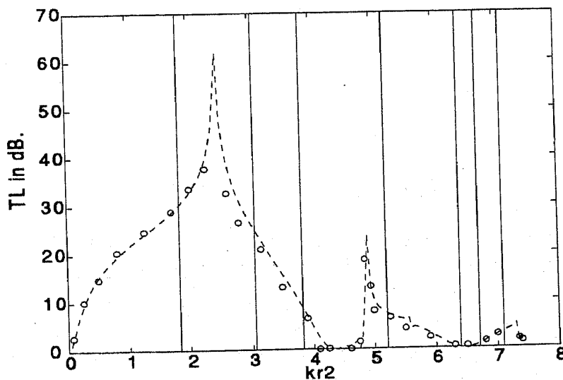
Figure 11. Comparison of the TL for a simple expansion chamber with d_1 = 0.0205 m, d_2/d_1 = 6 , l_2/d_2 = 0.33 , with the experimental results of Ih & Lee (1985) (- -) FEM, (o) experiments.
