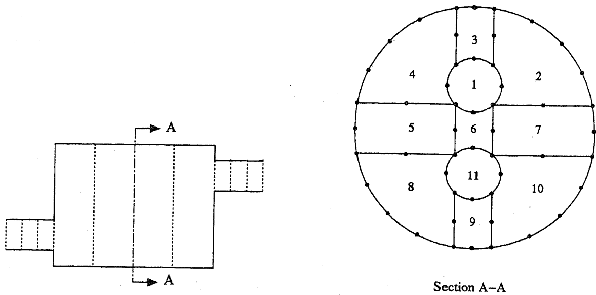
Figure 15. Discretized cross-section of an offset inlet/outlet model.
