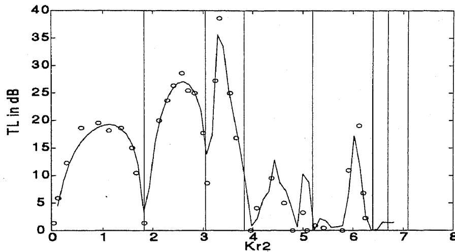
Figure 17. Comparison of FEM predictions (—) for an offset expansion chamber with the experimental results of Ih & Lee (1985). \alpha = 6 , \beta = 0.33 ; r_1 = r_3 = 10.25 mm; \delta_1 = \delta_2 = 0.37r_2 ; \theta = 180^\circ .
