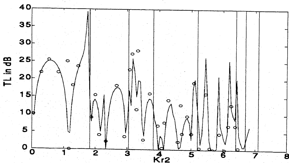
Figure 16. Comparison of the FEM predictions (—) for an offset expansion chamber with the experimental results of Ih & Lee (1985). \alpha = 6 , \beta = 1.35 ; r_1 = r_3 = 10.25 mm; \delta_1 = \delta_2 = 0.37r_2 ; \theta = 180^\circ .
