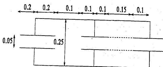
Figure 19. Extended tube expansion chamber in series with a concentric tube resonator.
