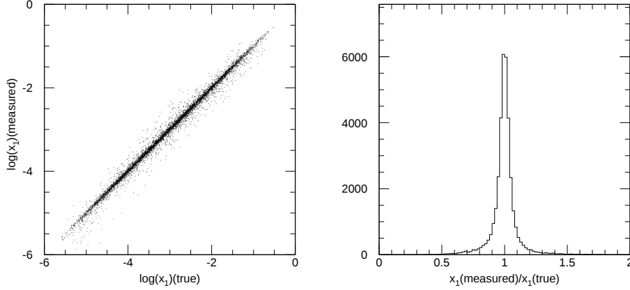
Figure 9: Left plot: correlation of the reconstructed value of \log(x_1) with the generated value for a sample of events passing the analysis requirements. Right plot: distribution of the ratio of the reconstructed and generated value of x_1 . The distributions are given for a sample of events passing the analysis cuts.
