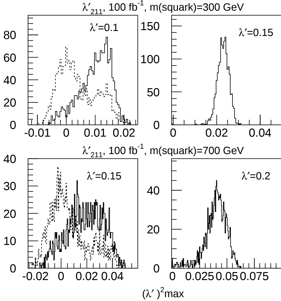
Figure 5: Distribution of the \lambda'_{211} value estimated through the maximization of the likelihood function for a set of \sim 1500 Monte Carlo experiments. The upper (lower) set corresponds to a squark mass of 300 (700) GeV. For each case, we show the distributions for three values of \lambda' used in the generation of events: 0 (dashed line), a value below the experimental sensitivity for the assumed squark mass and integrated luminosity (left plot, full line), and a value for which a good \lambda measurement is achievable (right plot). The integrated luminosity is 100 \text{ fb}^{-1} .
