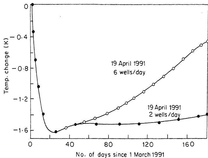
Figure 8. Surface cooling over Pakistan (for capping two and six wells per day starting from 19 April).
