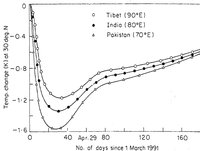
Figure 6. Surface cooling over Pakistan, India and Tibet (for capping three wells per day starting from 30 March 1991).
