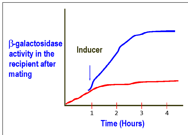
Figure 3. The PaJaMo experiment.
