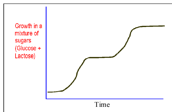
Figure 1. Diauxic growth curve.
