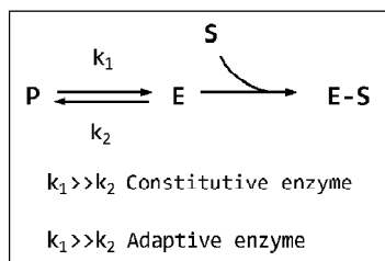
Figure 2. Adaptive versus constitutive enzymes.
