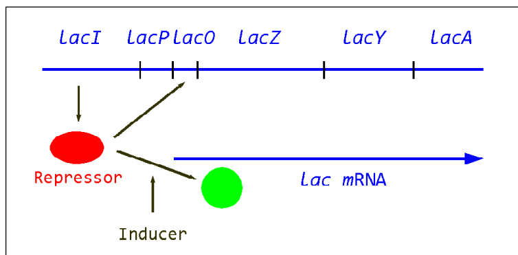
Figure 4. The lactose operon.
