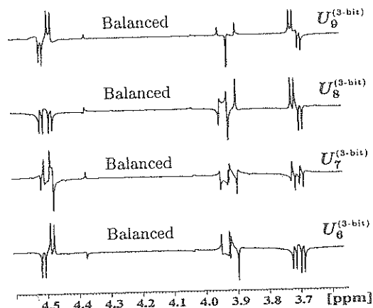
Figure 5. Entangling balanced functions implemented on the three-qubit system of 2,3-dibromopropionic acid.
