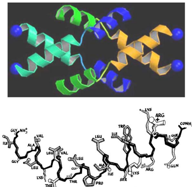
Fig. 2 X-ray crystal structure of melittin tetramer in solution at 2 Å resolution (top) (PDB code 2MLT). Each melittin monomer is composed of two \alpha -helical segments and the overall shape is that of a ‘bent rod’. Conformation of one melittin chain from the tetramer is shown below (Terwilliger and Eisenberg, 1982)
