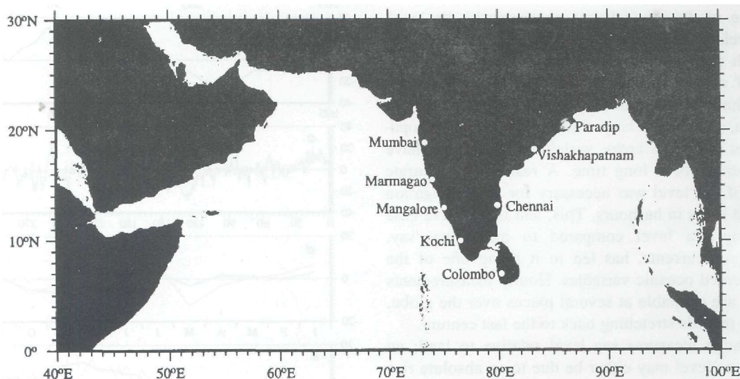
Figure 2. Tide gauge stations along the coast of the Indian subcontinent.
