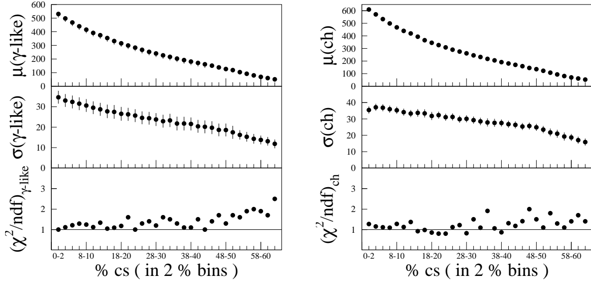
FIG. 4. Gaussian fit parameters of the multiplicity distributions of \gamma -like clusters and charged particles as a function of centrality. The centrality selection has been made by selecting 2% bins in minimum bias cross section, viz. , 0 – 2%, 2 – 4%, 4 – 6%, ..., 62 – 64%. The multiplicity distributions for these centrality bins are near perfect Gaussians as can be seen from the \chi^2/ndf values.
