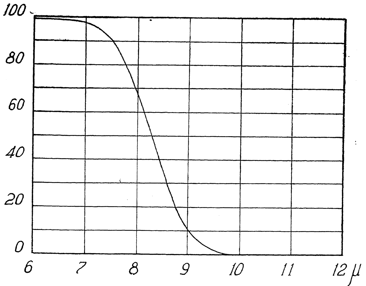
FIG. 1. Transmission by Fluorite; thickness 37 mm.
