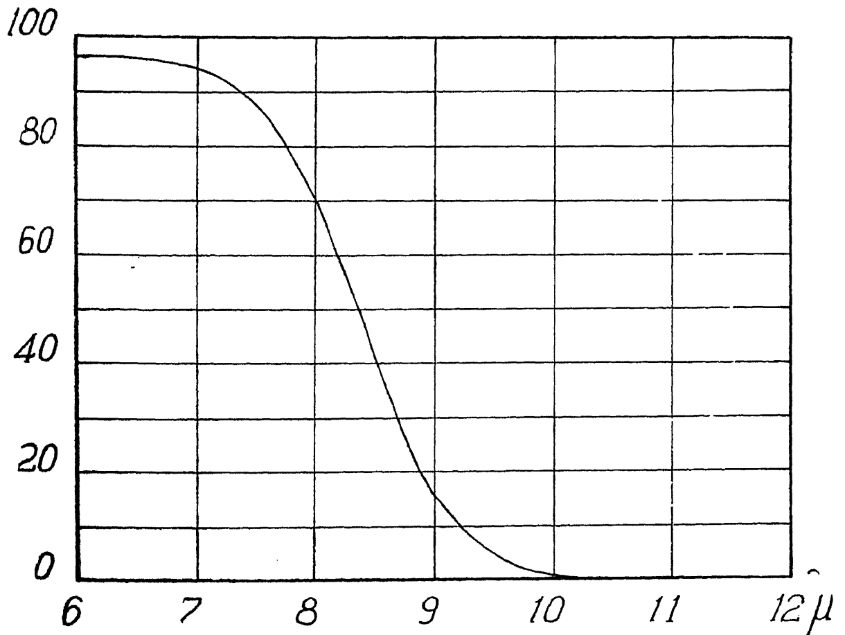
FIG. 2. Transmission by Fluorite; thickness 29 mm.
