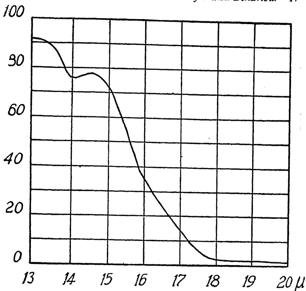
FIG. 9. Transmission by Fluorite; thickness 0.09 mm.
