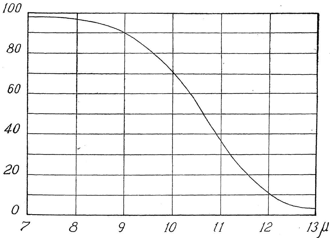
FIG. 5. Transmission by Fluorite; thickness 1 mm.
