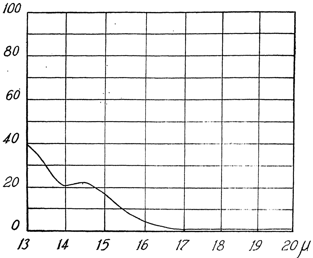
FIG. 7. Transmission by Fluorite; thickness 0.30 mm.
