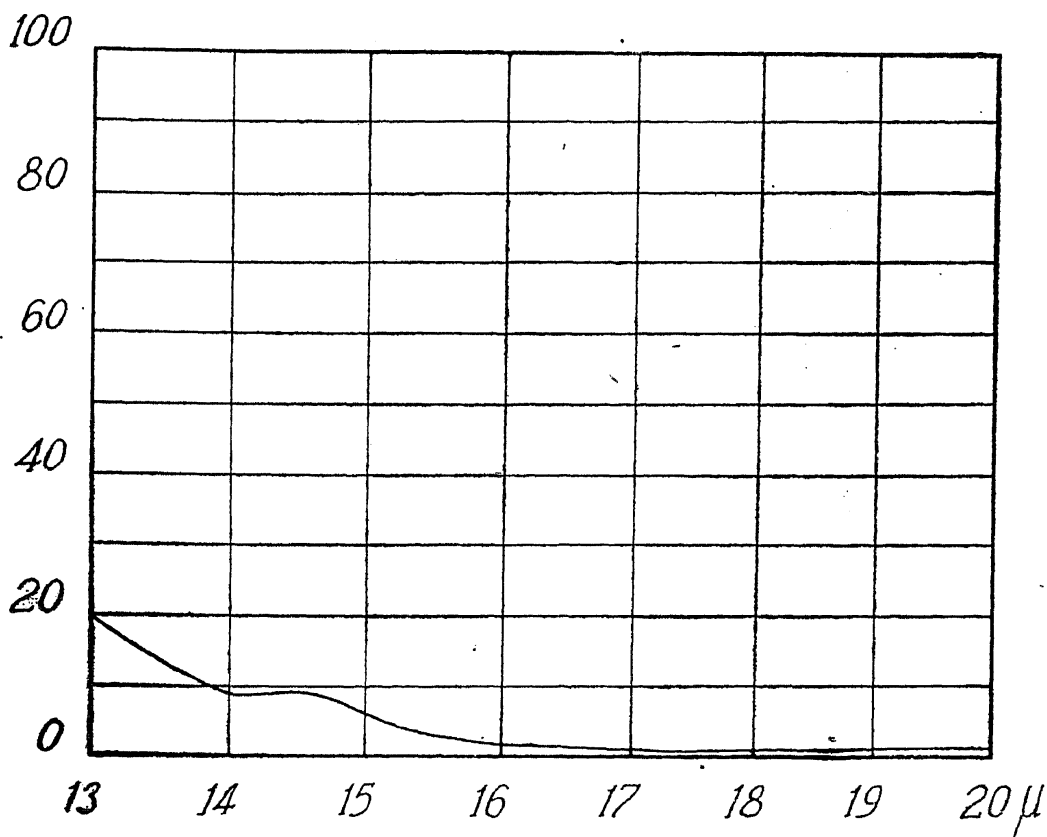
FIG. 6. Transmission by Fluorite; thickness 0.38 mm.
