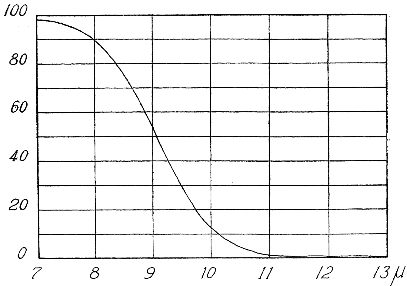
FIG. 3. Transmission by Fluorite; thickness 9 mm.
