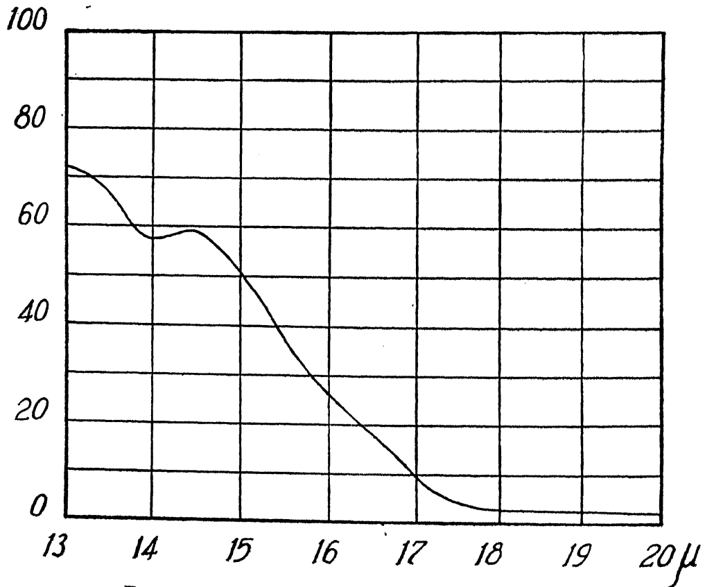
FIG. 8. Transmission by Fluorite; thickness 0.11 mm.
