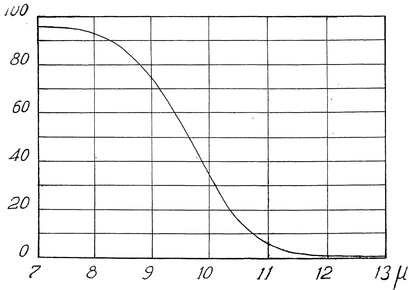
FIG. 4. Transmission by Fluorite; thickness 4 mm.
