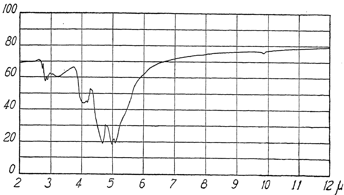
FIG. 2. Infra-Red Transmission of Group B Diamond (Thickness 1.06 millimetre).
