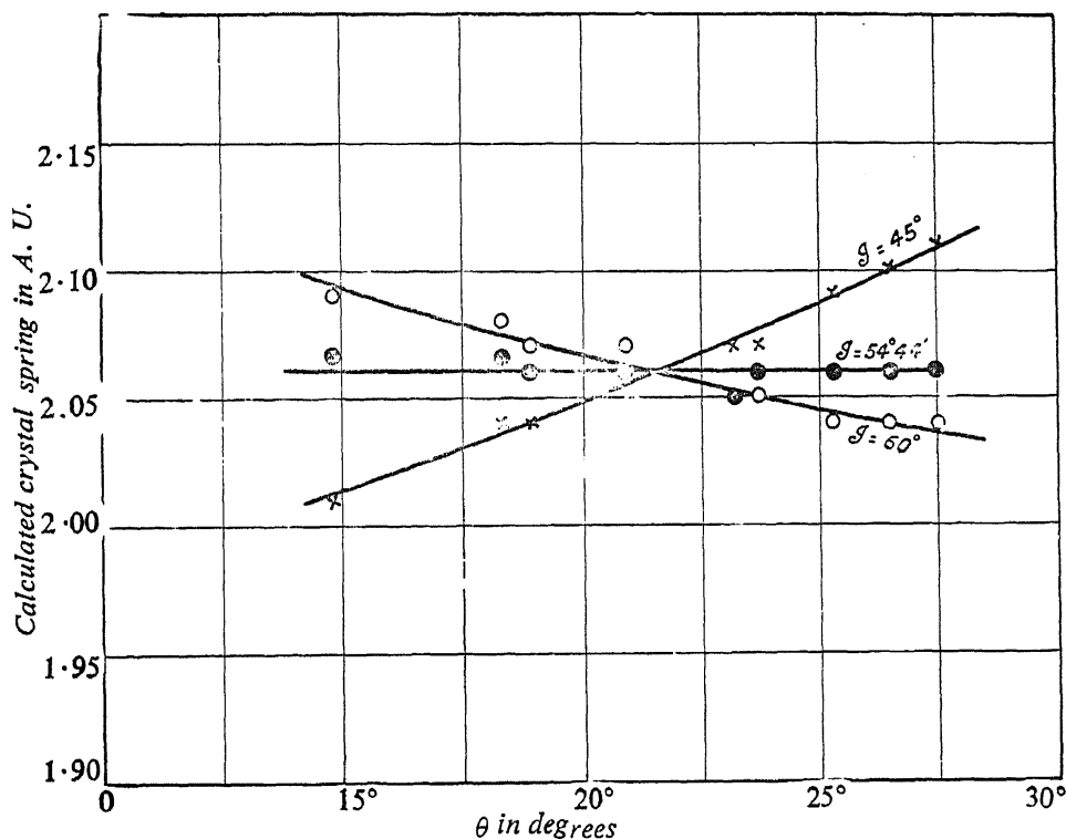
FIG. 4. Coincidence of Phase Waves in Diamond with Cubic Planes (After Raman and Nilakantan, November 1940)
