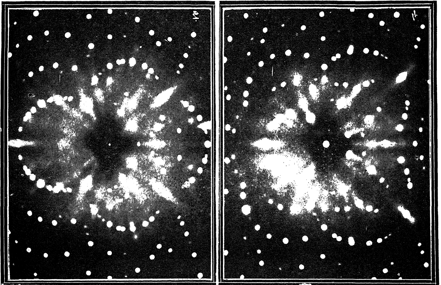
FIG. 10. Dynamic X-Ray Reflections by Calcite for Different Settings
