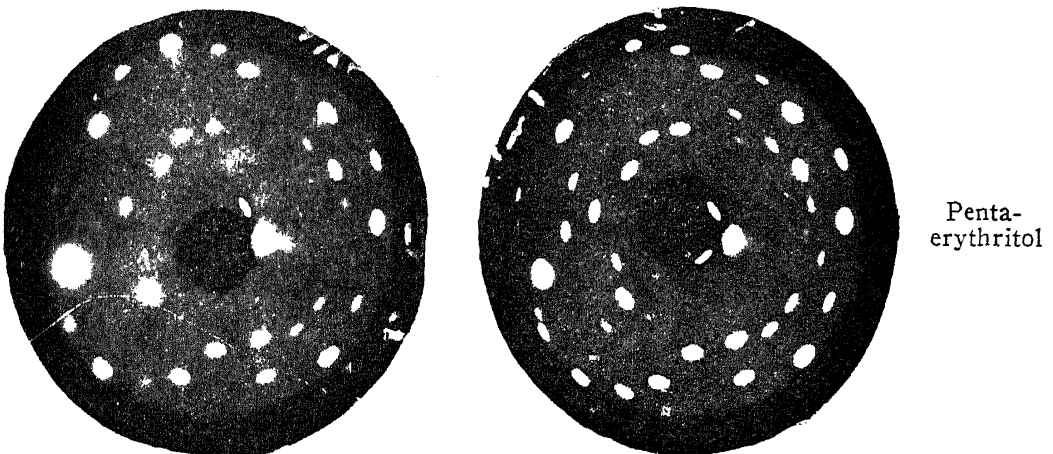
FIG. 6. Quantum X-Ray Reflections by Crystals at 30°C. (Left) and -180°C. (Right) (After C. S. Venkateswaran, September 1941)
