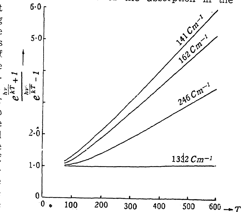
FIG. 7. Temperature Factor of Quantum Reflection, Theoretical (After Roman, September 1941)
