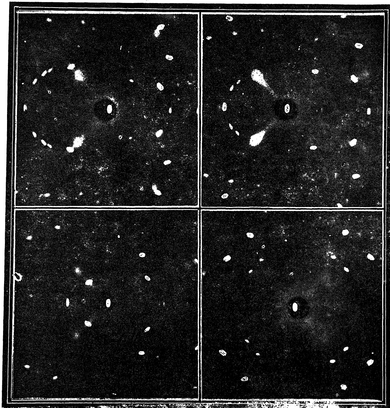
FIG. 9. Dynamic X-Ray Reflections by Hexamethyl Tetramine (After C. S. Venkateswaran, October 1941)
