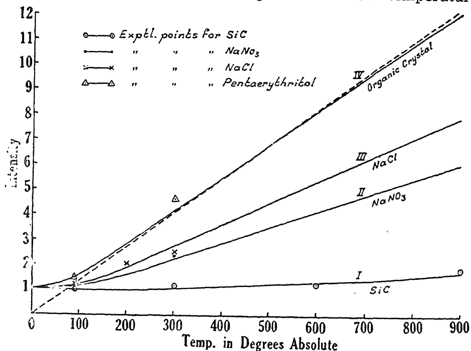
FIG. 8. Temperature Factor of Quantum Reflection, Experimental (After C. S. Venkateswaran, September 1941)
