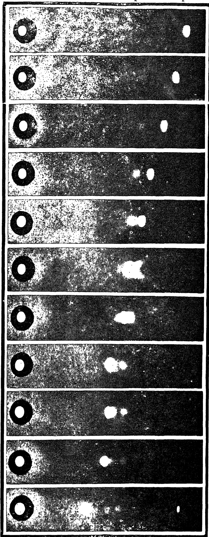
FIG. 3. Sequence of Changes in (111) Reflections by Diamond with Alteration of Crystal Setting (After Raman and Nilakantan, November 1940)
