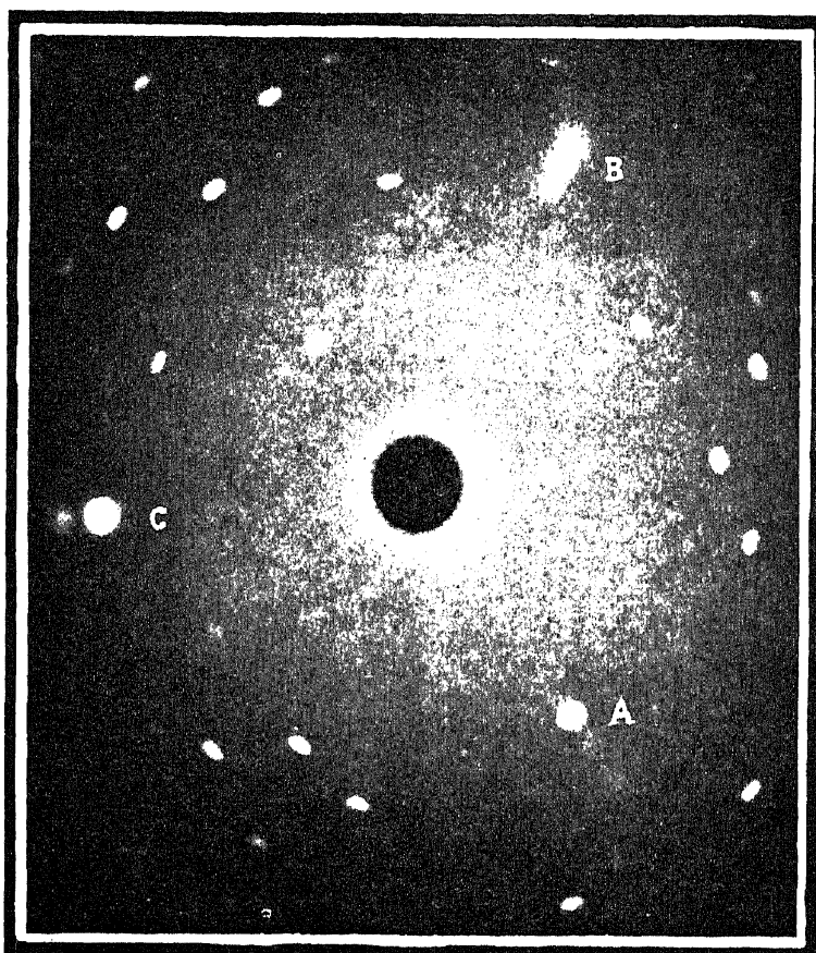
FIG. 2. Dynamic X-Ray Reflections by Diamond. \text{CuK}\alpha and \text{K}\beta Radiations (After Raman and Nilakantan, April 1940)
