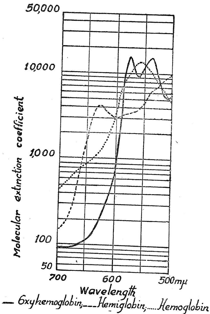
FIG. 4. Molecular Extinction Coefficients of Heme Pigments.
