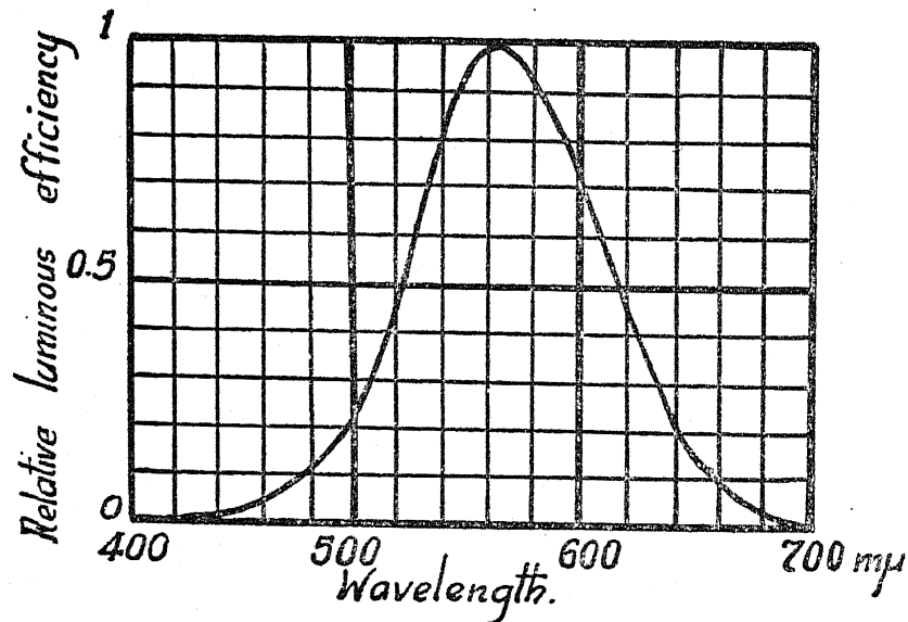
FIG. 2. Luminous Efficiency in the Spectrum.
