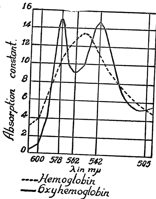
FIG. 3. Absorption Curves of the Blood Pigments.
