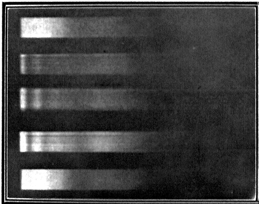
FIG. 1. Absorption spectrum of Aerules multiflorum with comparison spectrum. FIG. 2. Absorption spectrum of Clitoria Ternatea with comparison spectra.
