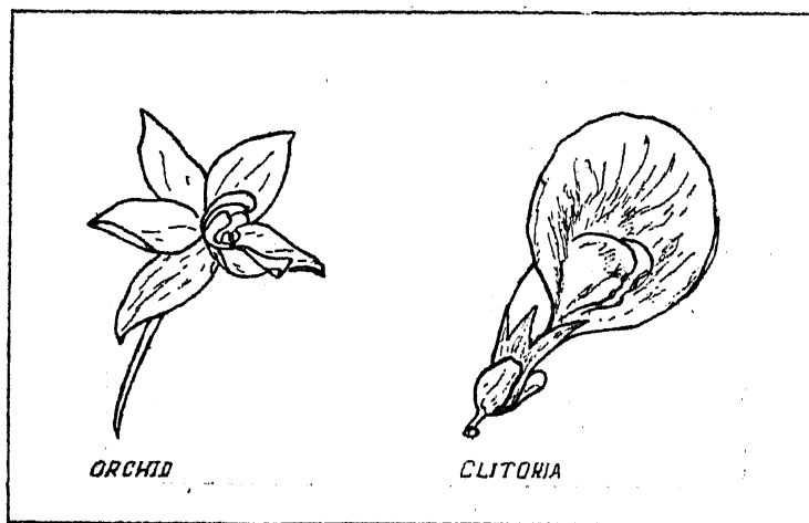
FIG. 1 (a) and (b). Flowers of Aerides multiflorum and Clitoria ternatea .
