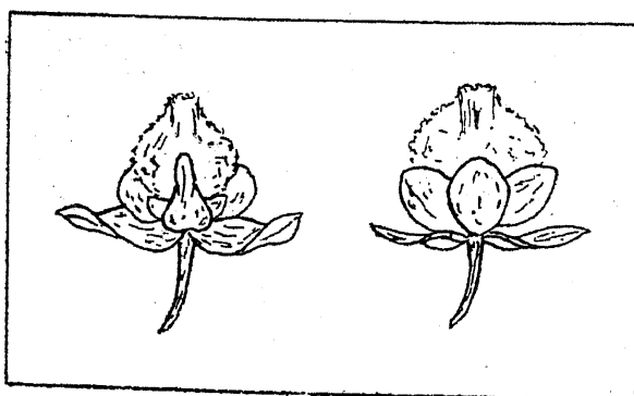
FIG. 2. Flower of Aerides crispum (front and back views).
