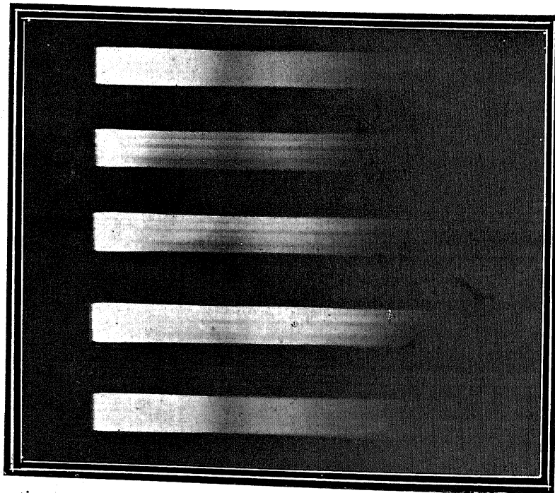
FIG. 1. Absorption spectrum of Peltorum ferrugineum with comparison spectra. FIG. 2. Absorption spectrum of Oxalis acetosella with comparison spectra.
