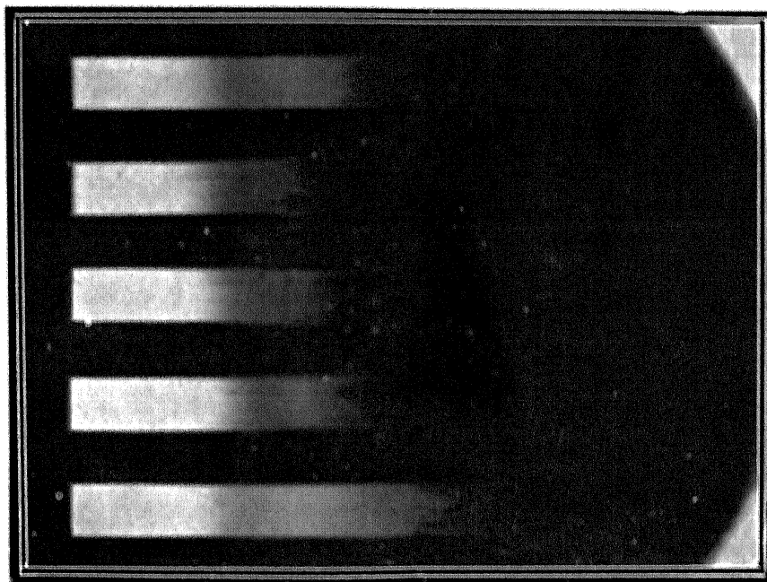
FIG. 1. Absorption spectrum of Allamanda grandiflora with comparison spectra.
