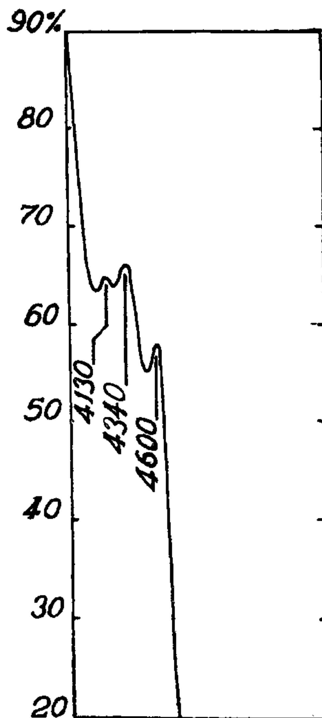
FIG. 2. Absorption spectrum of yellow rose.
