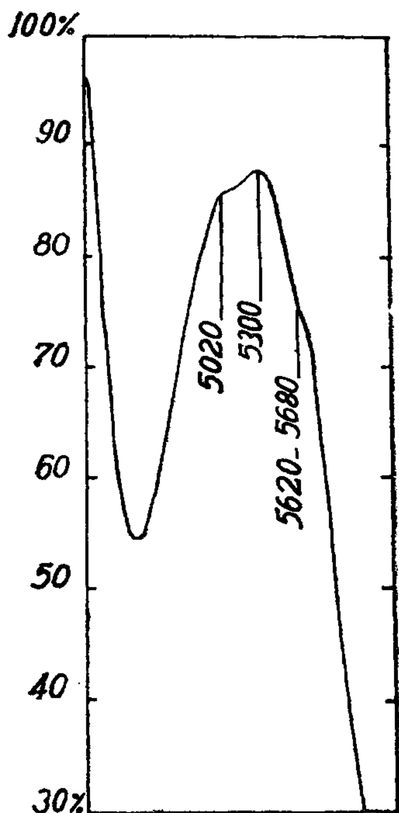
FIG. 1. Absorption spectrum of red rose.
