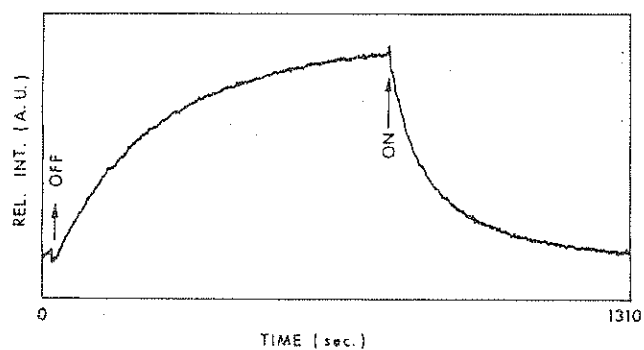
Figure 9. Decay kinetics of and recovery of Fe^{3+} signal in E1 (under uniform illumination).
