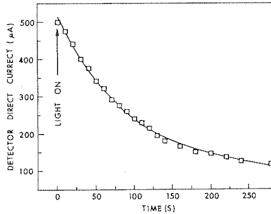
Figure 7. Time dependent changes of the detector current with nonuniform illumination of M1 crystal.
