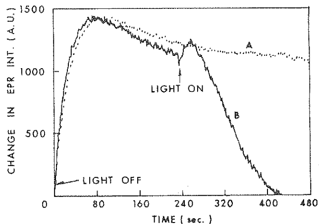
Figure 8. Kinetics of decay and recovery of Fe^{3+} signal in M1 (under uniform laser illumination).
