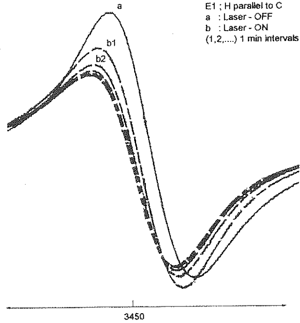
Figure 5. Effect of He-Ne laser illumination on the 1/2 \leftrightarrow -1/2 line of Fe^{3+} in E1.
