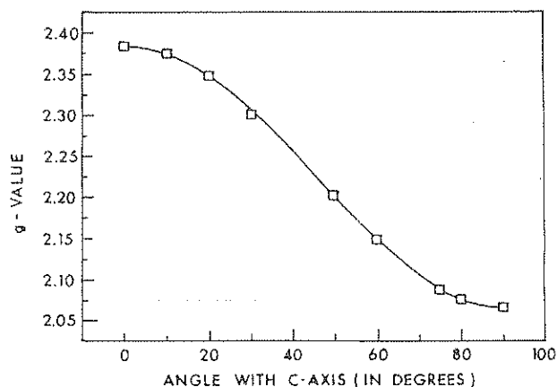
Figure 4. Angular variation of the g -tensor for \text{Cu}^{2+} in \text{BaTiO}_3 (MI). The solid line is theoretical line and the points are experimental points.
