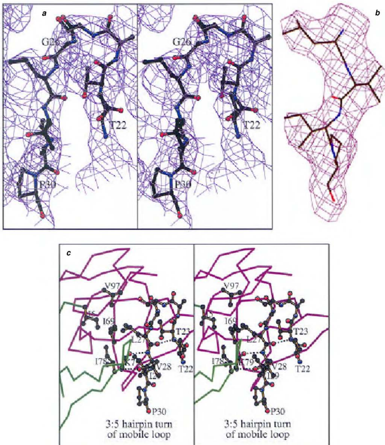
Figure 2. Conformation of the mobile loop. a , Stereoview of the omit map calculated by omitting the mobile loop and the neighbouring 5 Å residues from structure factor calculations. The \sigma_A weighted difference maps are contoured 2 standard deviations above the mean value. The density clearly shows two antiparallel strands with a hairpin conformation. Electron density in all the seven monomers looked similar to the one shown here, suggesting similar conformation adopted by the mobile loop in all the seven subunits. The residues at the two termini of the loop, Thr22 and Pro30, as well as the conserved Gly26 are labelled. This figure was generated using Bobscrip 19 ; b , Electron density map of the conserved LVI sequence of Mt-cpn10 ; c , Interaction of mobile loop residues with the rest of the chaperonin-10 molecule shown in stereo. Leu27 and Ile29 of the conserved Leu-Val-Ile tripeptide are buried in the hydrophobic core formed by adjacent chaperonin-10 monomers. Other residues involved in the hydrophobic core are shown in ball-and-stick. C ^{\alpha} traces of two monomers are shown in different colours. The characteristic 3:5-turn hydrogen bond between Thr23 NH and Leu27 CO is indicated. The hydrogen bonds between the main chain groups of Val28 and Lys79 are also indicated.
