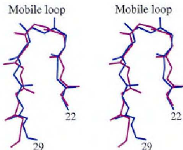
Figure 3. Superposition of the mobile loop \beta -turn of E. coli structure (magenta) and Mt -cpn10 (blue). The two flanking strands exhibit similar twist in the two structures. The figure was generated using MOLSCRIPT 20 .
