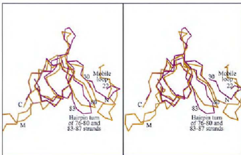
Figure 1. Superposition of M. tuberculosis (magenta) and E. coli (yellow) monomer structures. The \beta -hairpin from residues 76–87 undergoes a rigid body movement and exposes a hydrophobic patch that accommodates the mobile loop of the neighbouring subunit in the mycobacterial structure (see text for details). The mobile loop of the superposed subunit of E. coli structure ( M ) is also indicated for comparison. The N- and C-termini of the E. coli chaperonin-10 are indicated.
