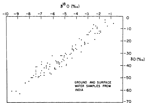
Figure 4. Plot of \delta D versus \delta^{18}O for water samples for which both the measurements were done. The data show that these two variables are linearly related (see text).
