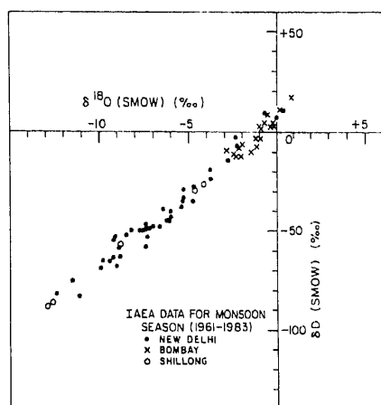
Figure 5. Plot of \delta D versus \delta^{18}O for rain-water samples collected during monsoon season (June to September) from three Indian stations showing a linear relation between these two variables. The data are taken from IAEA reports.
