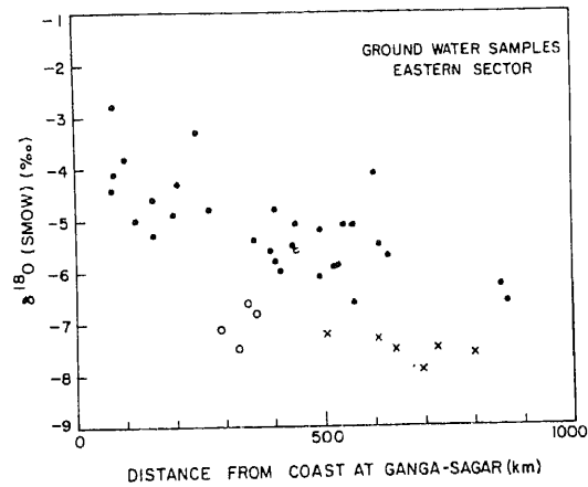
Figure 2. \delta^{18}O values of the groundwater samples collected east of Lucknow (sample numbers 22 to 57 and A1 to A4 in table 1) as a function of the distance of the sampling locations from the nearest coastal point (taken as Ganga Sagar). x—samples taken from places close to big rivers and irrigation systems; o—samples taken from higher altitudes.
