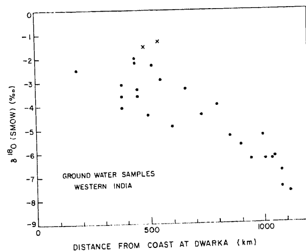
Figure 3. \delta^{18}O values of the groundwater samples, collected west of Lucknow (sample numbers 58 to 80) and some locations from Gujarat, as a function of the distance of the sampling locations from the nearest coastal point (taken as Dwarka). x—samples unusually enriched (see text).
