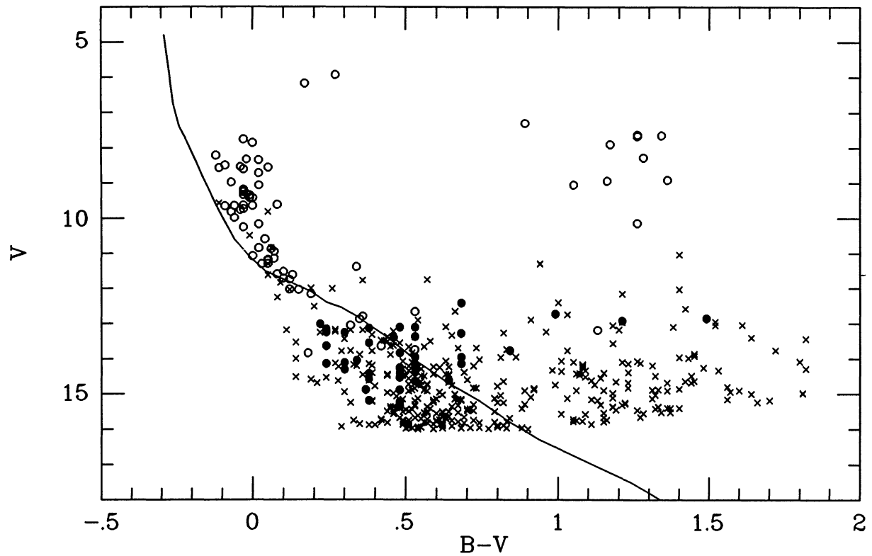
FIGURE 7. A ( V , B - V ) colour-magnitude diagram for NGC 3114 based on photoelectric observations ( \circ ) from the literature and CCD observations from Table 2 ( \times ). The stars in the spectroscopic sample which have B magnitudes determined via photographic photometry and B - V colours from spectral classification are shown using the \bullet symbol. The solid line shows the fitted ZAMS (see text).
