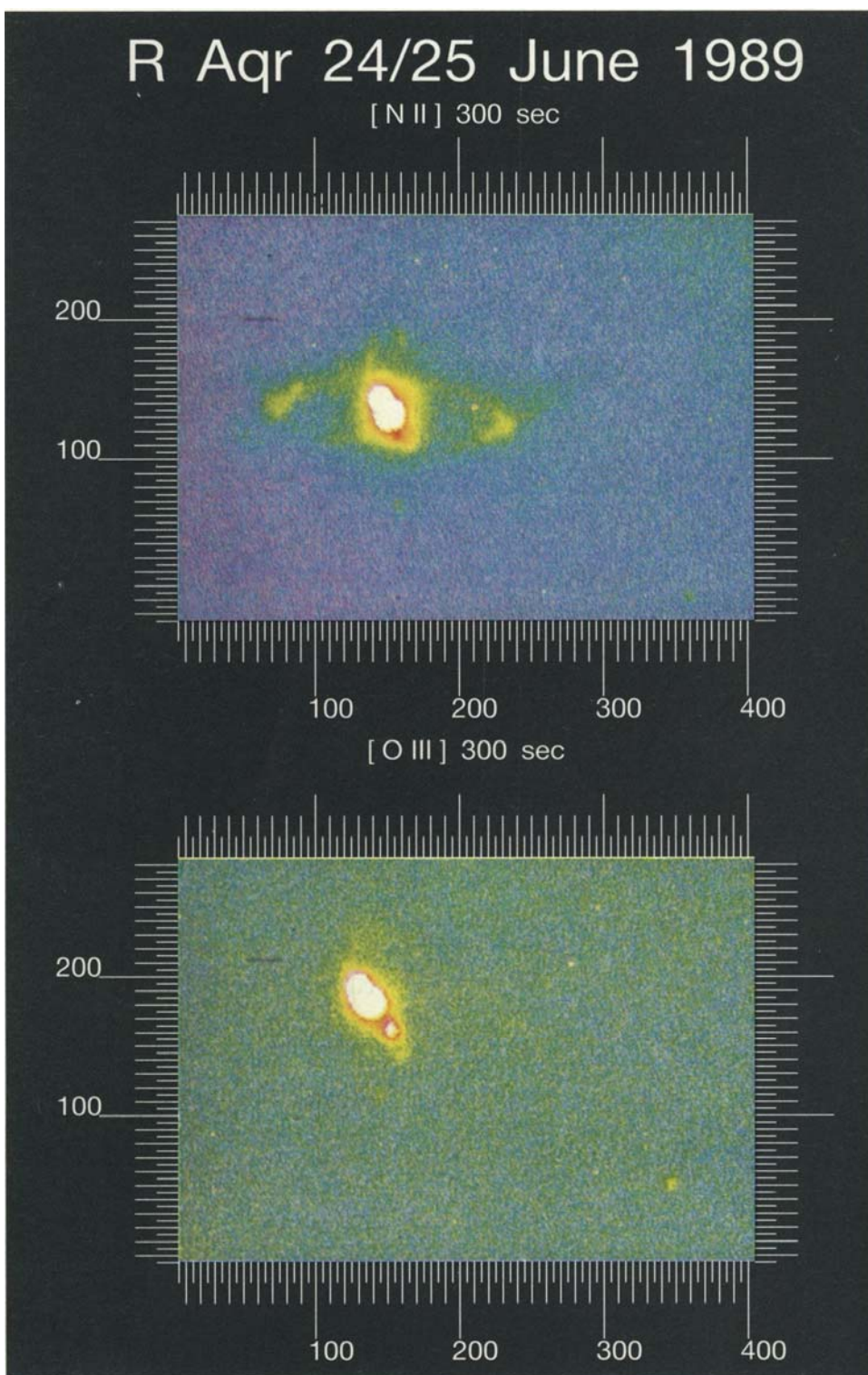
Figure 3. Colour picture of the faint nebulous features of R Aqr. Orientation and other notations are the same as in Fig. 1.
