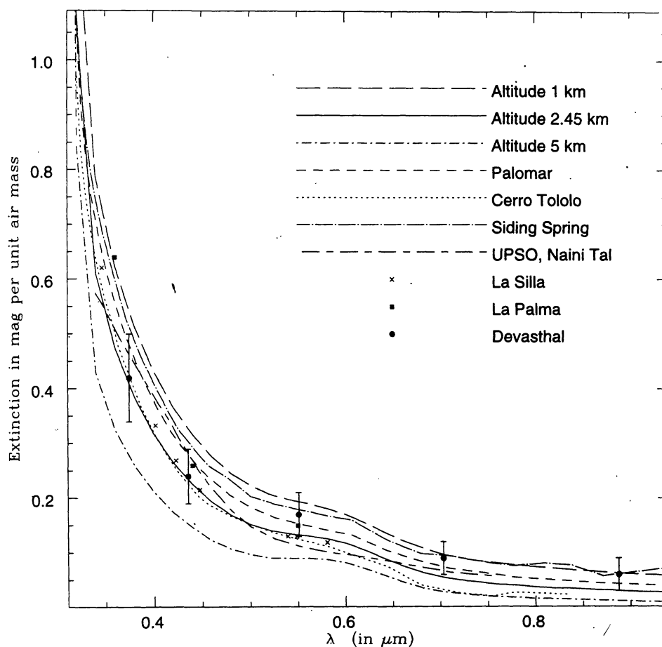
Figure 1. A comparison of the Devasthal's average atmospheric extinction law with those at Siding Spring in Australia, La Silla and Cerro Tololo in Chile, La Palma in Spain, Palomar in USA and UPSO, Naini Tal in India. Total extinction expected due to molecular absorption, Rayleigh and aerosol scatterings by molecules and particles present in the Earth's atmosphere for sites located at altitude of 1, 2.45 and 5 km are also shown.
