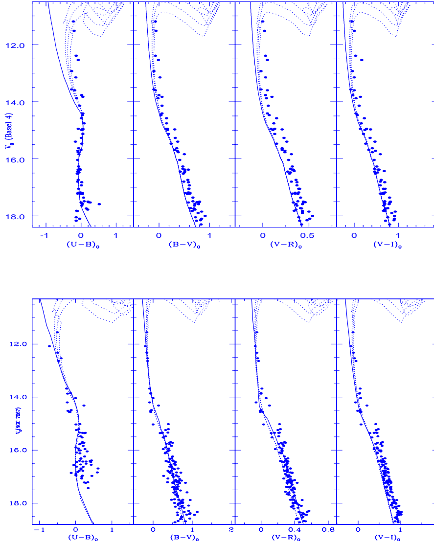
Figure 9. The V_0, (U - B)_0 ; V_0, (B - V)_0 ; V_0, (V - R)_0 and V_0, (V - I)_0 diagrams for stars of the Basel 4 and NGC 7067. The continuous curves, ZAMS fitted to the MS and dotted curves are the isochrones for Z = 0.008 stars of \log(\text{age})=8.2, 8.3 and 8.4 for Basel 4 and Z = 0.02 stars of \log(\text{age})=7.9, 8.0 and 8.1 for NGC 7067.
